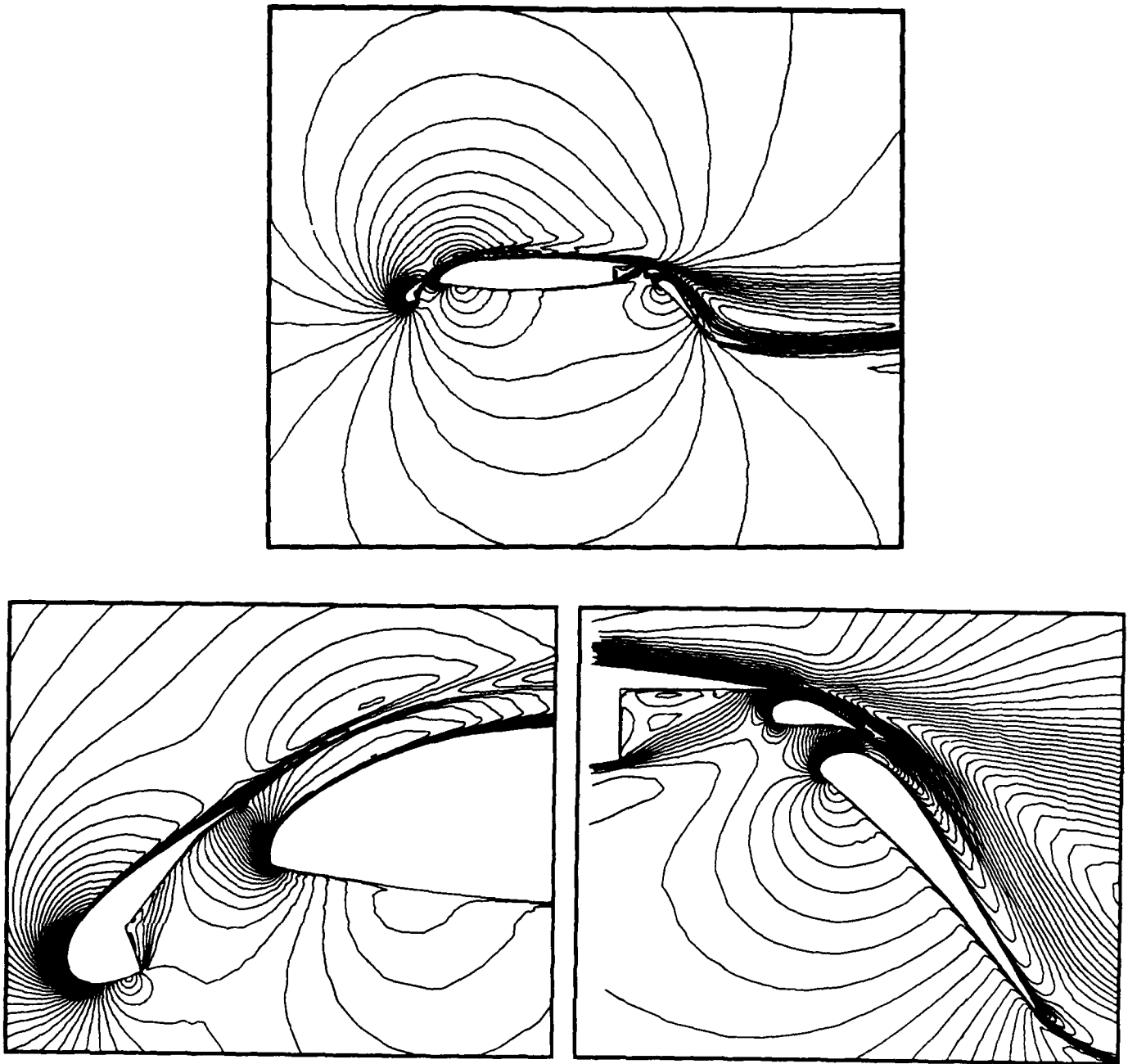
Figure 17 Computed Mach Contours for Flow over Four-Element Airfoil Mach = 0.1995, Reynolds Number = 1.187 million, Incidence = 16.02 degrees
