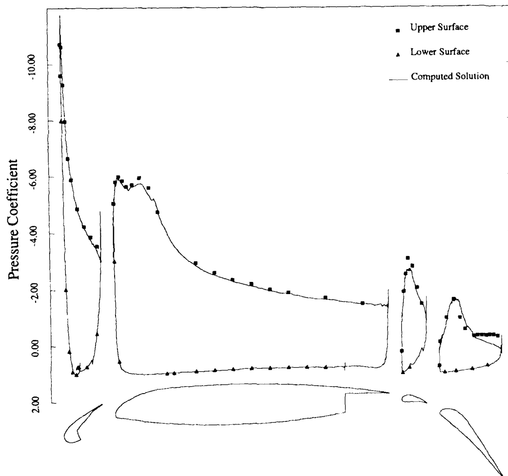
Figure 18 Comparison of Computed Surface Pressure Distribution with Experimental Wind-Tunnel Data for Flow Over Four-Element Airfoil Configuration Mach = 0.1995, Reynolds Number = 1.187 million, Incidence = 16.02 degrees
