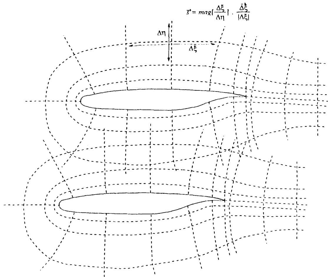
Figure 1 Overlapping Structured C-Meshes for Multi-Element Airfoil Geometry Providing Initial Definition of Mesh-Point Distribution and Local Stretching Factors
