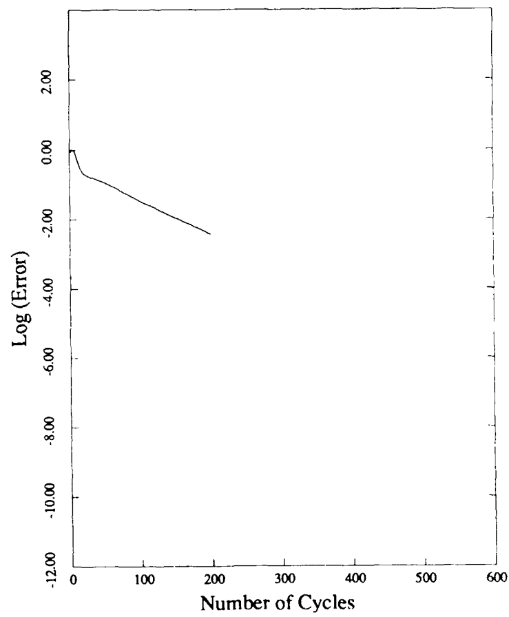
Figure 15 Convergence Rate as Measured by RMS Average of the Density Residuals Versus the Number of Multigrid Cycles for Flow Past a Two-Element Airfoil
