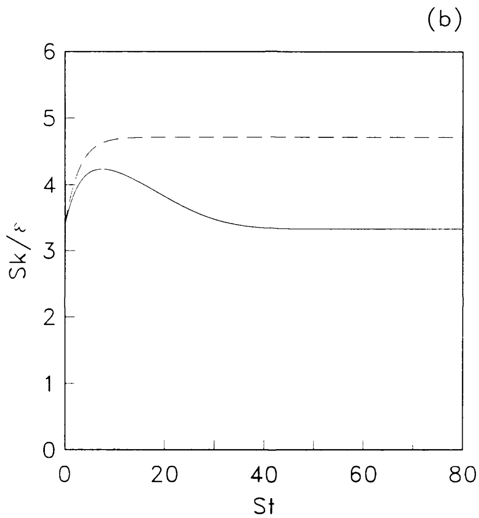
Figure 7. Comparison of the model predictions for Sk/\epsilon : — S_K^{(c)} = 0.01 ; - - - standard k - \epsilon model. (a) Short time solution, and (b) long time solution.
