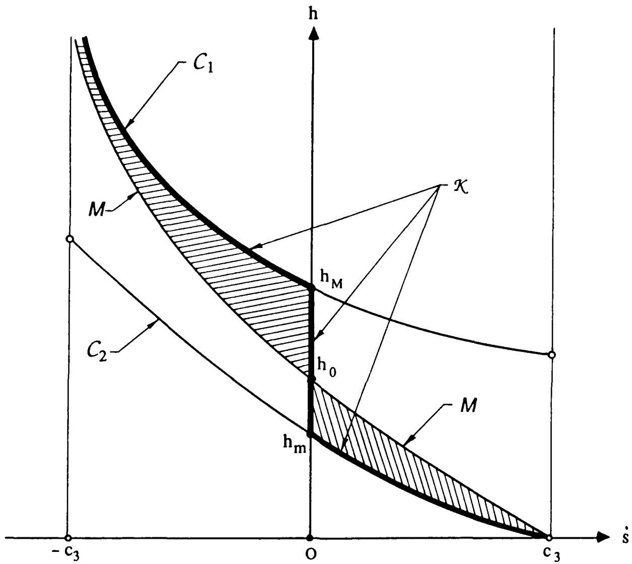
FIGURE 8. THE CURVE \kappa IN THE \dot{s}, h -PLANE CORRESPONDING TO SOLUTIONS OF THE RIEMANN PROBLEM SELECTED BY THE MAXIMALLY DISSIPATIVE KINETIC RELATION.
