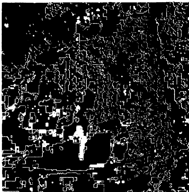
Figure B8. Classification Map for DIRS Enhancement 2 (30 m hybrid)
