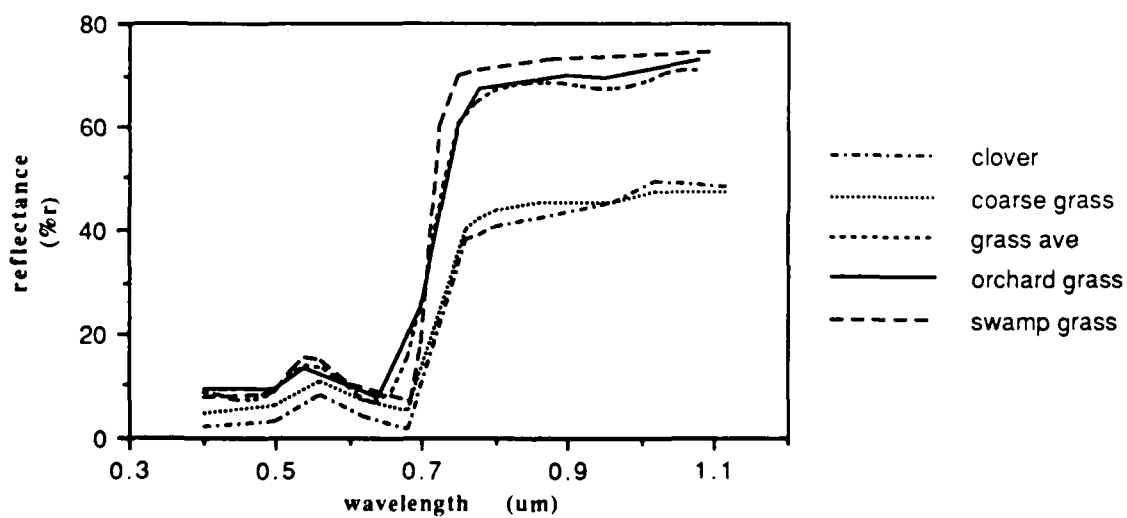
Figure 2-6 Reflectance Spectra of Selected Grass Targets
