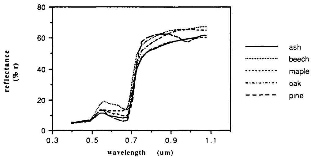
Figure 2-5 Reflectance Spectra of Selected Tree Targets
