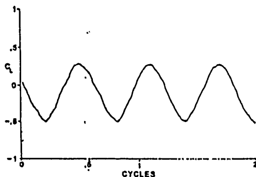
Fig. 13 Unsteady pressure and lift coefficients produced by an auto-rotating flat plate 0.5c upstream of a stationary airfoil at 0^\circ ; 3" flat plate, left - Re 50,000, right - Re 100,000; effective reduced frequency 1.6 and 1.8 for Reynolds numbers of 50 and 100 K .
