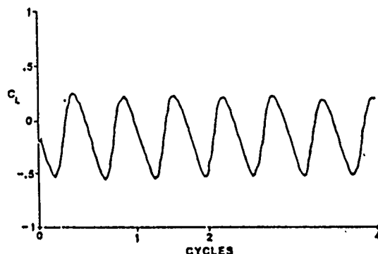
Fig. 13 Unsteady pressure and lift coefficients produced by an auto-rotating flat plate 0.5c upstream of a stationary airfoil at 0^\circ ; 3" flat plate, left - Re 50,000, right - Re 100,000; effective reduced frequency 1.6 and 1.8 for Reynolds numbers of 50 and 100 K .
