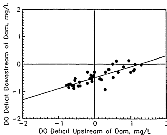
Fig. 1. Aeration at New Cumberland Lock and Dam, Ohio River.
