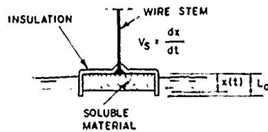
FIGURE 1 - SOLUBLE SOLID FLOAT GENERAL ARRANGEMENT AND DETAIL
