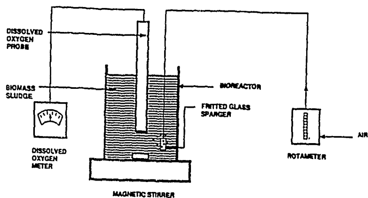
FIGURE 1. BIOLOGICAL SYSTEM WITH A BUBBLE COLUMN.
