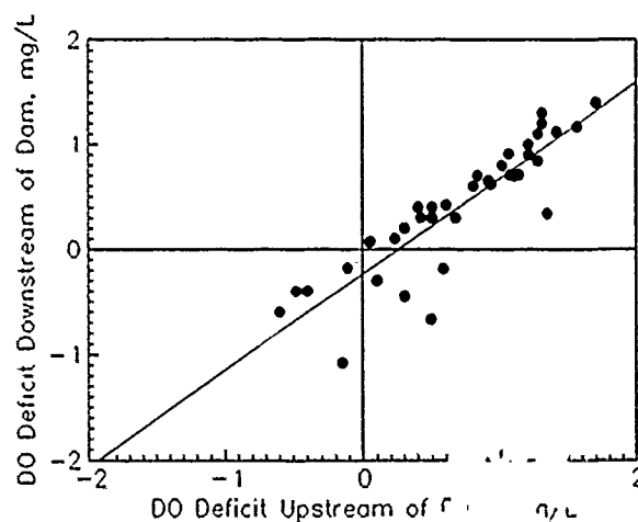
Fig. 2. Aeration at Hannibal Lock and Dam, Missouri.
