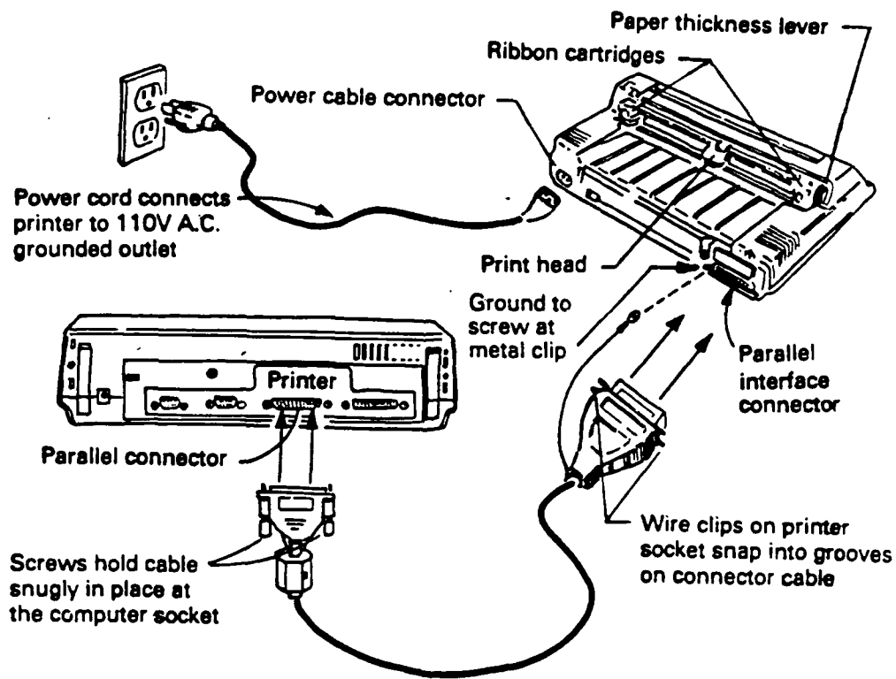
Figure 1-8. Connecting the printer cable.
