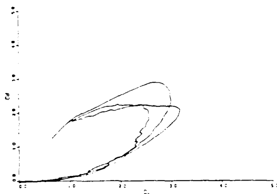
Figure 17 C_d vs C_l , Cases IV, VI, VII
