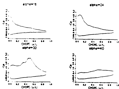
Figure 8 C_p vs x/c , Case VII
