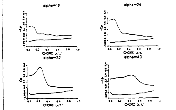
Figure 14 C_p vs x/c , Case VI
