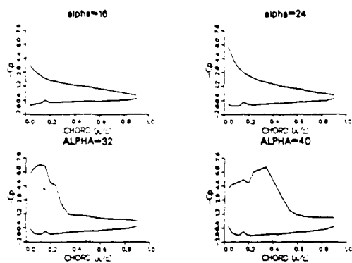
Figure 15 C_p vs x/c , Case VII
