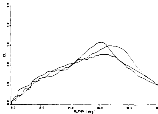
Figure 16 C_l vs alpha, Cases IV, VI, VII
