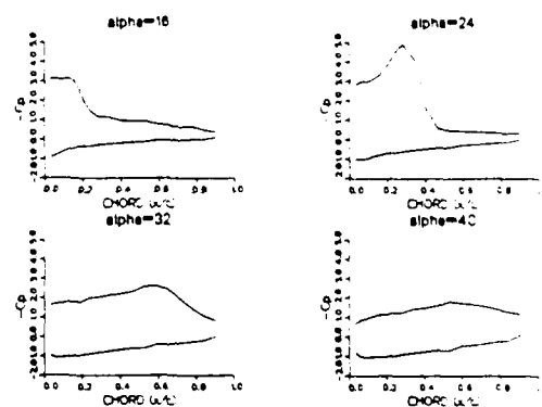
Figure 7 C_p vs x/c , Case III
