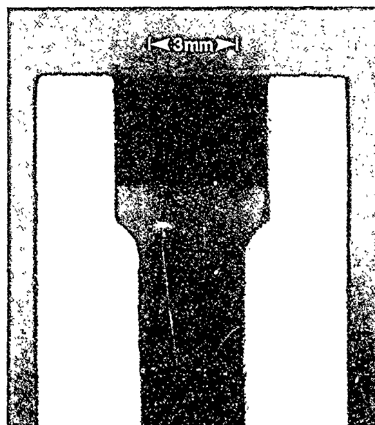
Figure 20 Detail of Dynasen Inc. carbon gauge for low stress measurements (1-2 GPa). Refer to Horning and Isbell (1975) for a discussion.
