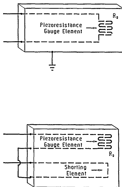
Figure 30 Schematic showing electrical corrections required for noise created from inductive pick-up (Tokheim, 1986).
