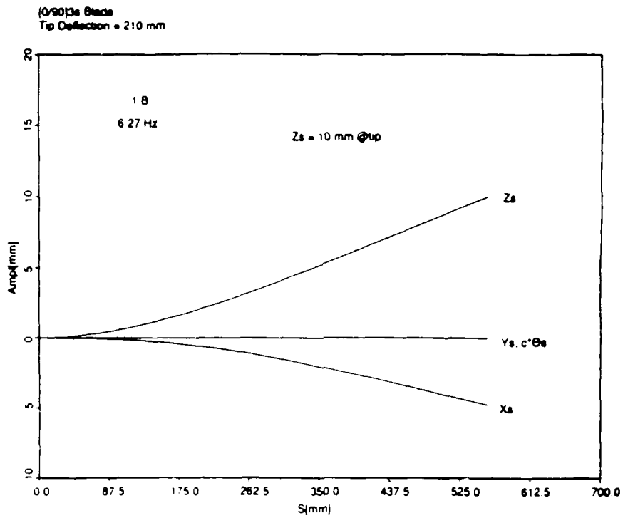
Figure 19: First Bending Mode; (0/90) 3s , 210 mm tip deflection, Zs=10 mm
