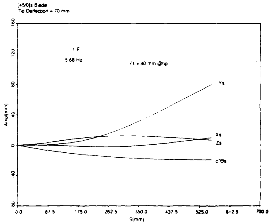
Figure 47: First Fore-and-Aft Mode;[45/0] s ,70 mm tip deflection,Ys=80 mm
