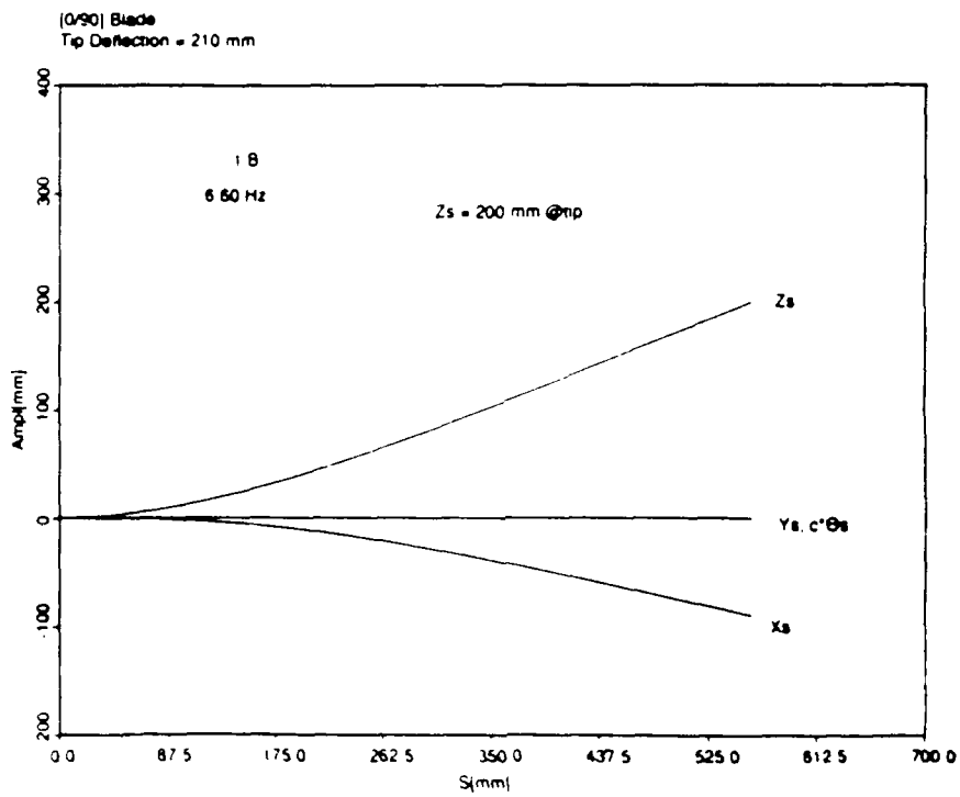
Figure 20: First Bending Mode; (0/90) 3s , 210 mm tip deflection, Zs=200 mm
