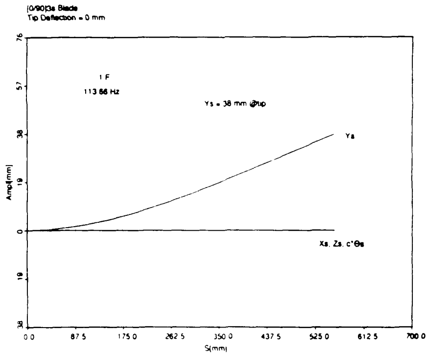
Figure 8: First Fore-and-Aft Mode:[0/90] 3s ,0 mm tip deflection, Y_s=38 \text{ mm}
