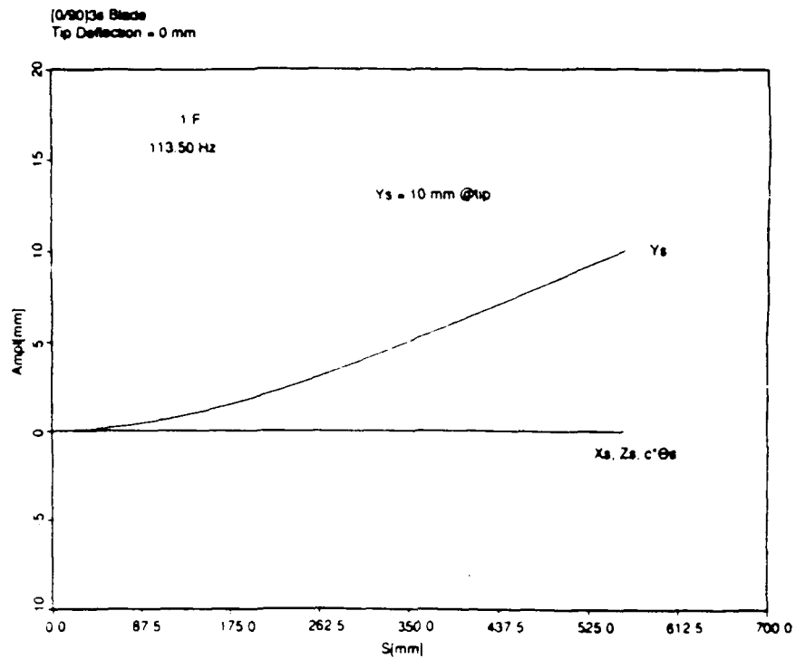
Figure 7: First Fore-and-Aft Mode:[0/90] 3s ,0 mm tip deflection, Y_s=10 \text{ mm}
