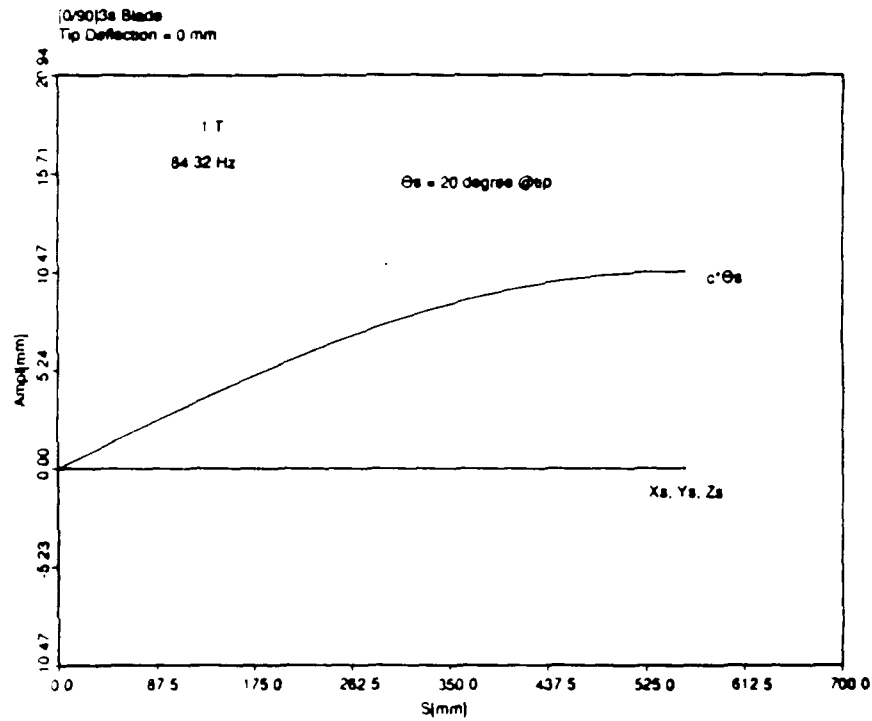
Figure 10: First Torsion Mode;[0/90] 3s ,0 mm tip deflection, \theta_s = 20 \text{ degree}
