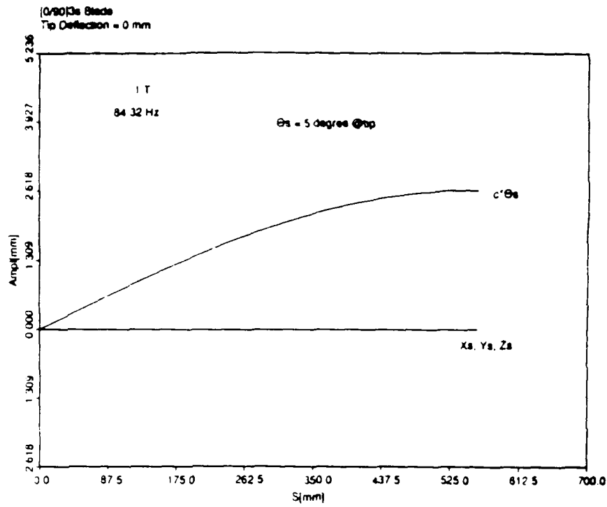
Figure 9: First Torsion Mode;[0/90] 3s ,0 mm tip deflection, \theta_s = 5 \text{ degree}
