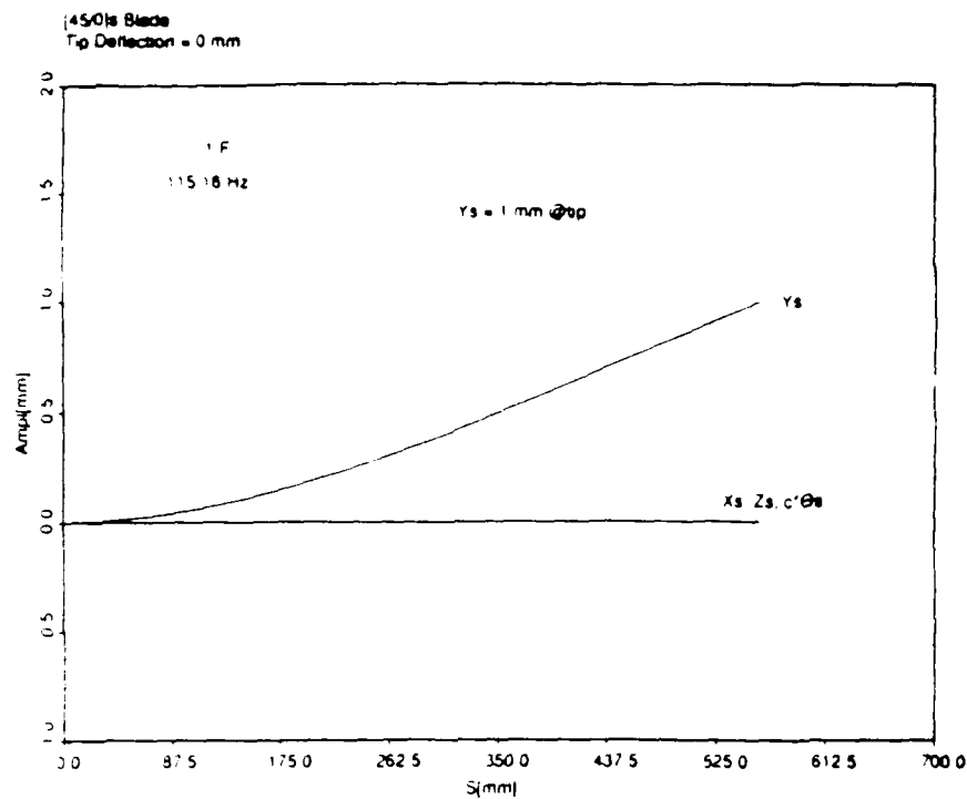
Figure 38: First Fore-and-Aft Mode;[45/0]s,0 mm tip deflection,Ys= 1 mm
