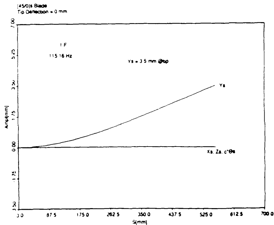
Figure 39: First Fore-and-Aft Mode;[45/0]s,0 mm tip deflection,Ys= 3.5 mm
