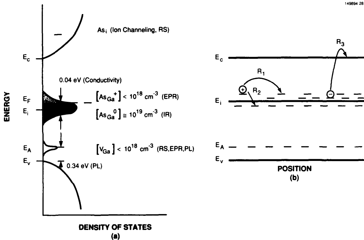
Figure 5-2. Preliminary model for LT GaAs annealed in situ at 600°C for 10 min illustrating (a) semiquantitative density of states and (b) band diagram. The techniques used to identify the defects are shown in parentheses in (a). PL indicates photoluminescence; RS indicates Raman scattering measurements; and R_1 , R_2 and R_3 refer to conduction mechanisms discussed in the text.
