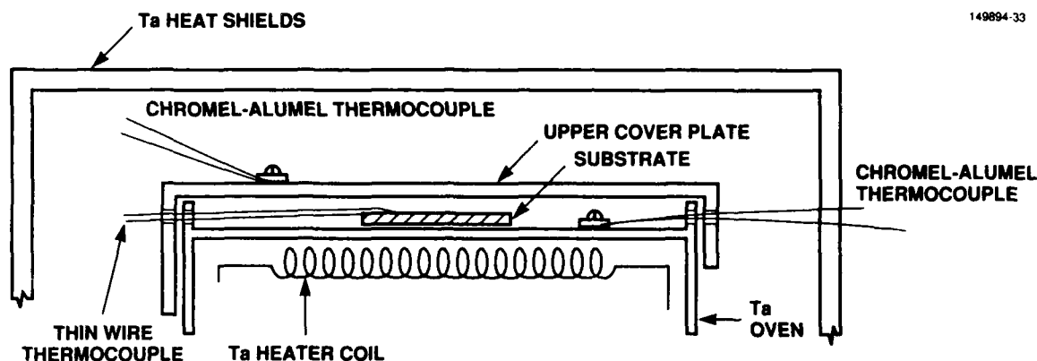
Figure 6-2. Vacuum oven for thermocouple calibration.
