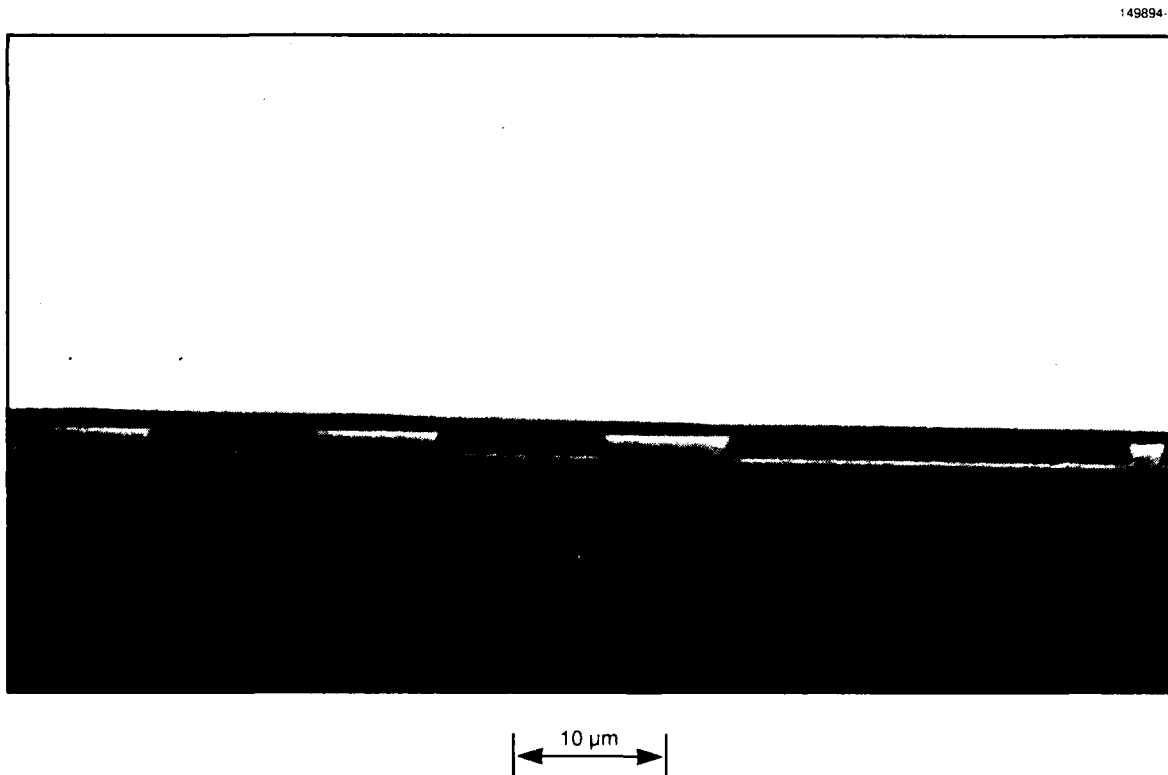
Figure 4-1. SEM of 1.5\text{-}\mu\text{m} -high \text{SiO}_2 steps planarized with a 2.5\text{-}\mu\text{m} -thick PECVD a\text{-C:H} film.
