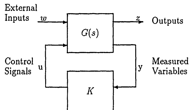
Figure 9.1: H^\infty System Representation.
