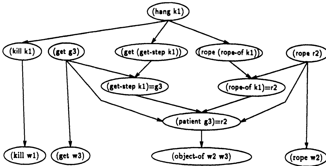
Figure 1: The Bayesian network for "Jack got a rope. He killed himself."
