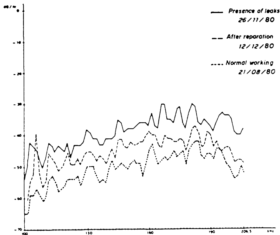
Figure III-8. Trending Spectra of Acoustic Emmission Transducer Indicating Leak Developing [Ref. 24]
