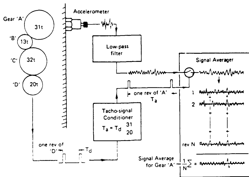
(a) Signal averaging applied to gearboxes
