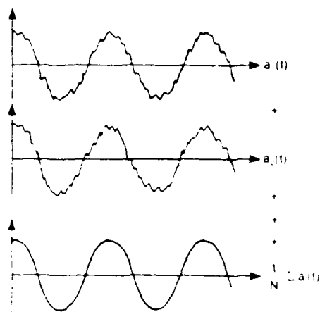
Figure IV-11. Synchronous Time Domain Averaging [Ref. 5]
