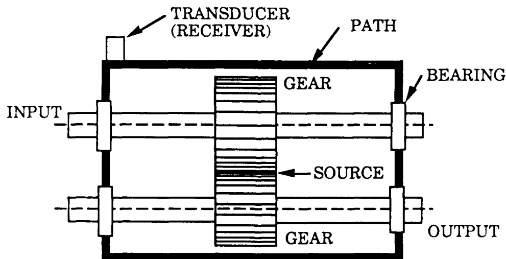
Figure IV-3. Source-path-receiver Model.
