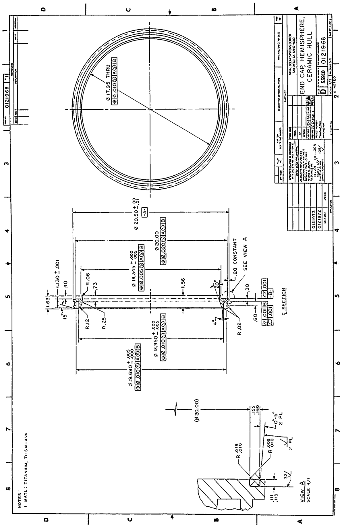
Figure 17. Fabrication drawing of Mod 0 end cap for 20-inch ceramic hemispheres.
