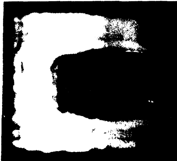
Fig. 4 -- The burn pattern made on run ML4 of 10 Jan. 1985. Direction of flow is from left to right.
