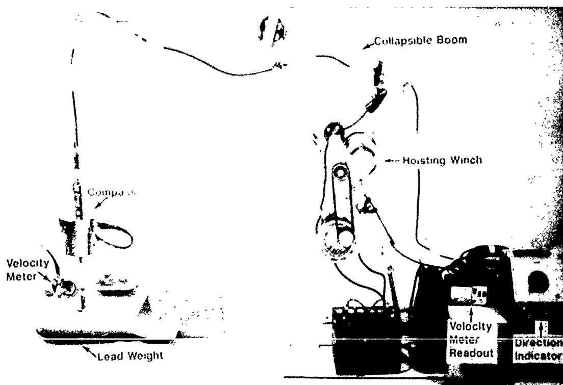
Figure 5. Over-the-side equipment
