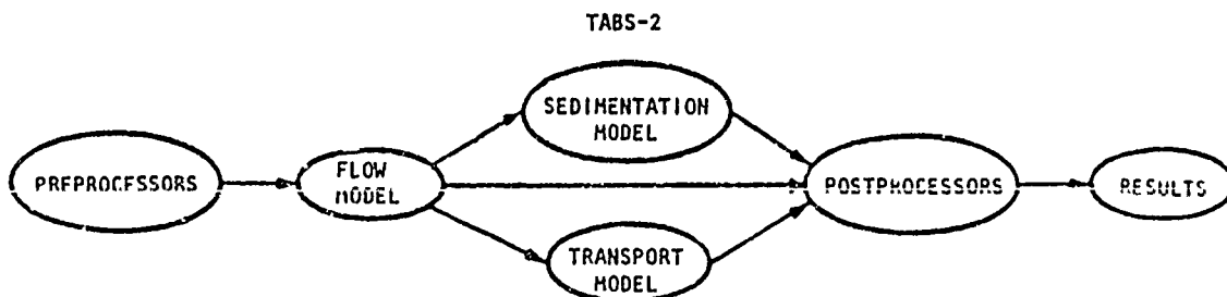
Figure B1. TABS-2 schematic
