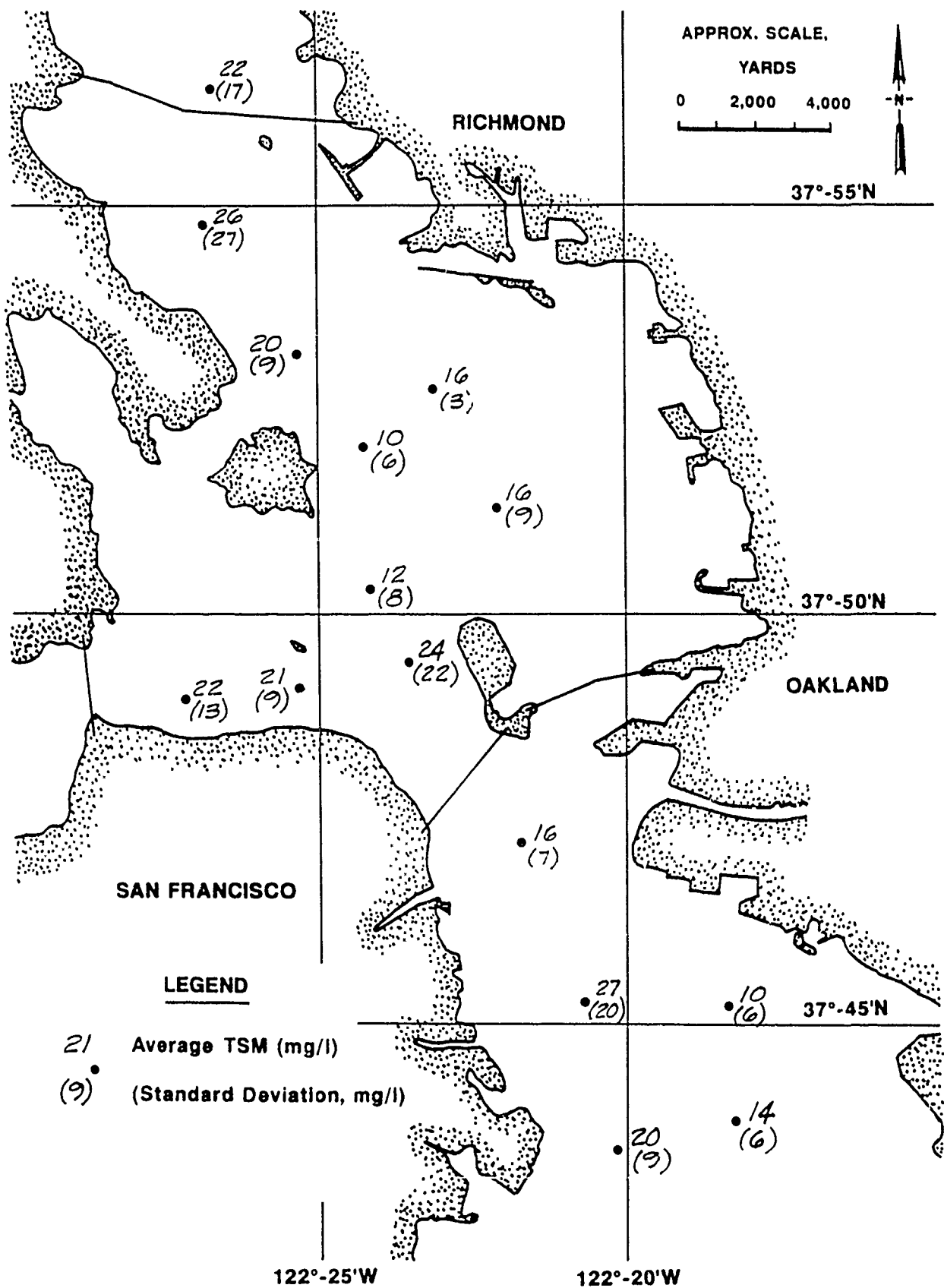
Figure 14. Point sample average TSM and standard deviations
