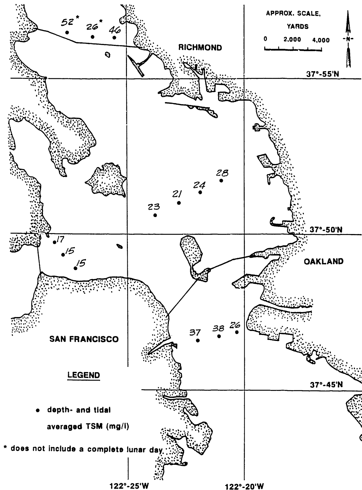
Figure 12. Depth- and tidal-averaged TSM values for the intensive survey
