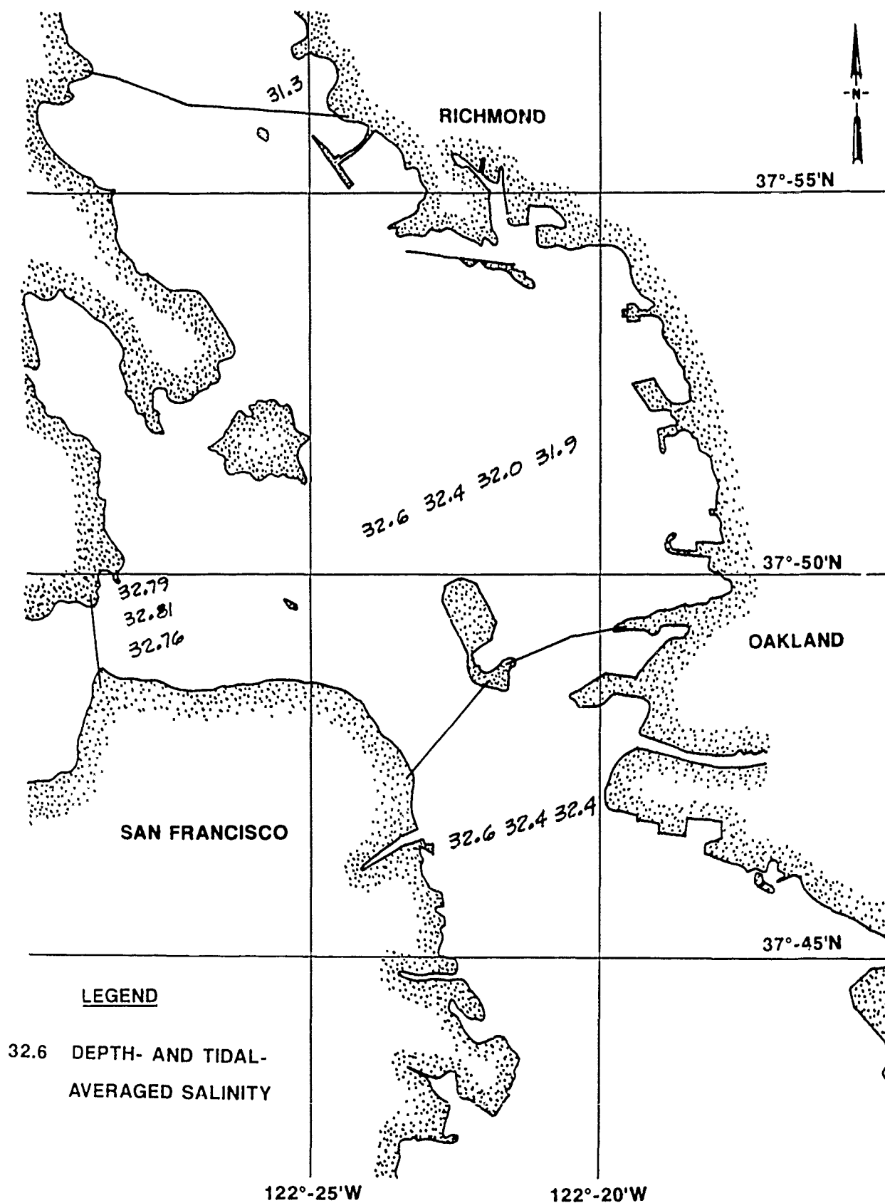
Figure 13. Depth- and tidal-averaged salinities for the intensive survey
