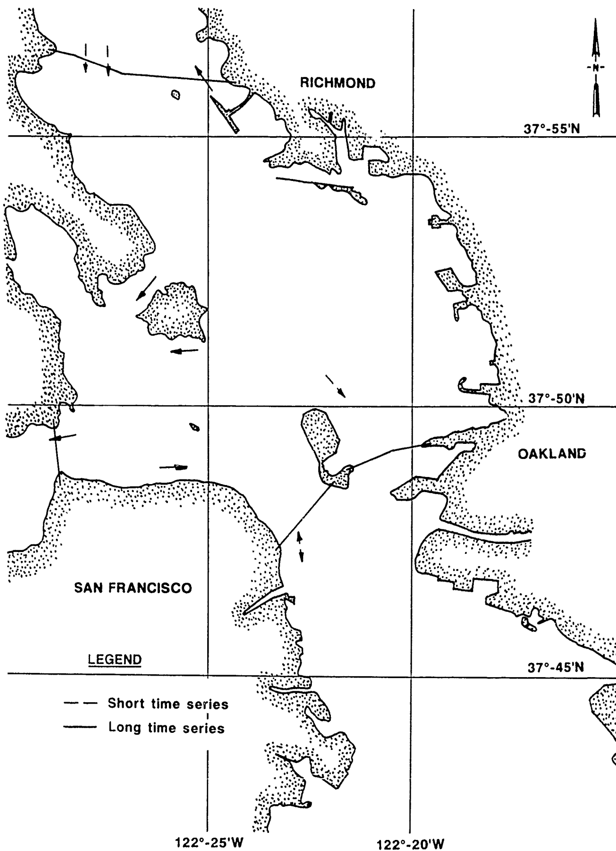
Figure 18. Tidal dominance of bottom currents
