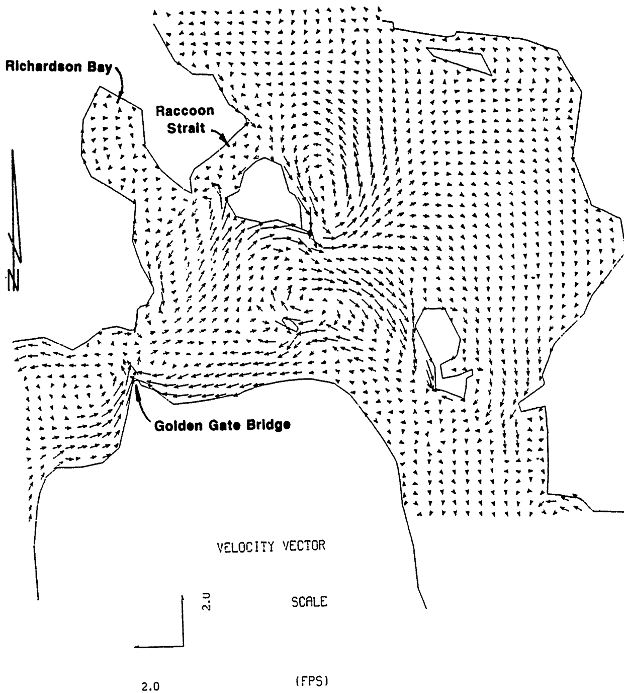
Figure 23. Numerical model predicted residual current pattern for central San Francisco Bay
