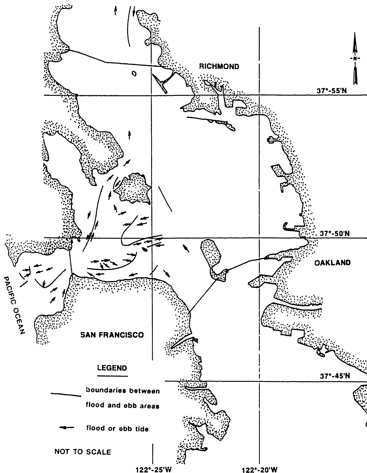
Figure 16. Direction of near-bottom current maximums
