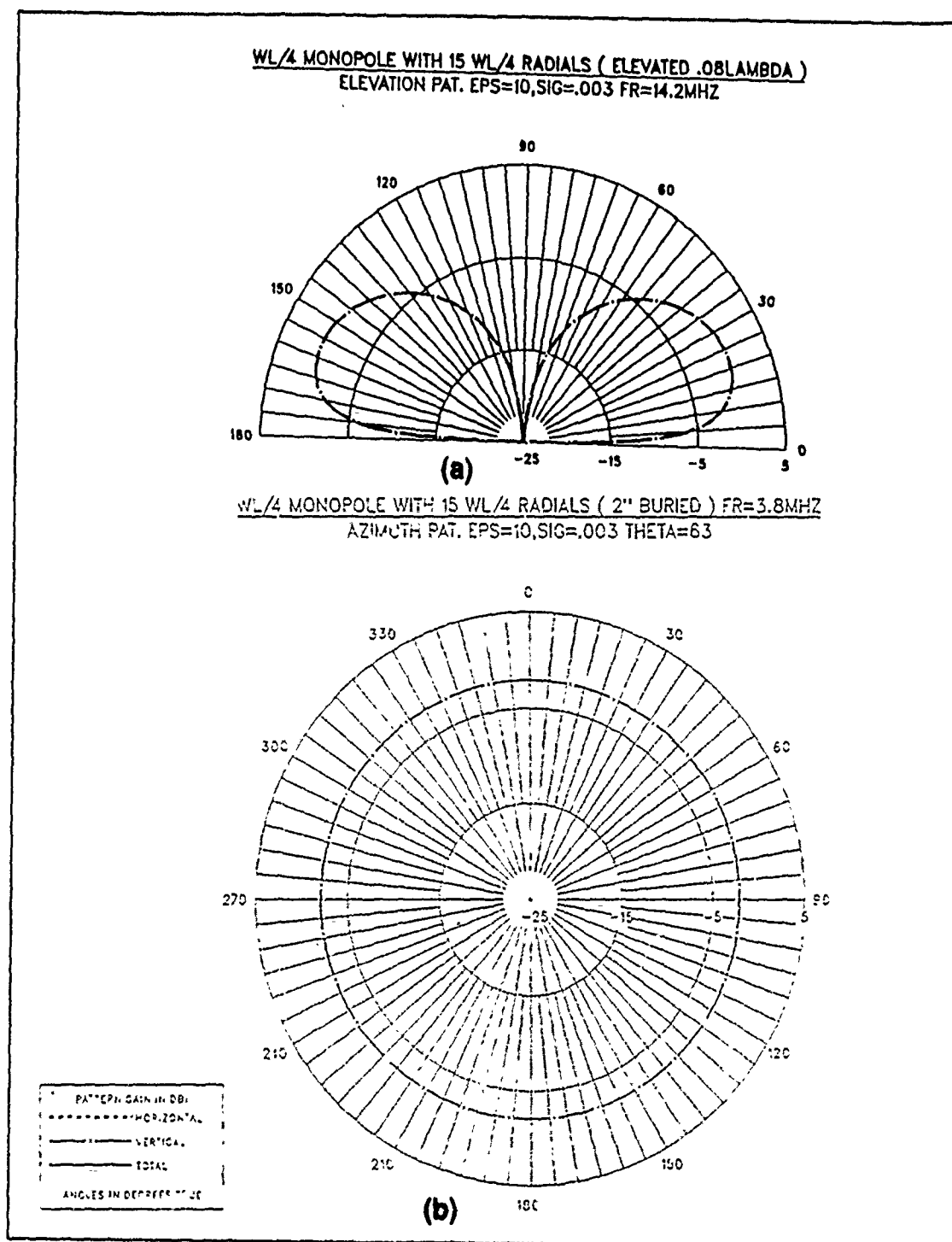
Figure 29. The radiation patterns of the monopole with elevated radials: (a) Elevation pattern (b) Azimuth pattern
