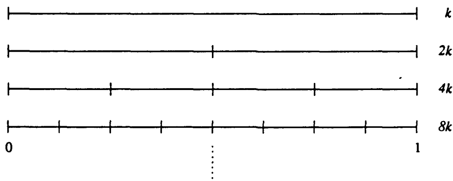
Figure 1.3: Multi-wavelet bases of \mathcal{L}^2[0, 1] consist of functions non-zero on intervals of various scales. The basis of order k contains k functions supported on each interval of one scale, which does not overlap other intervals of that scale. The total number of functions on a single scale is shown.
