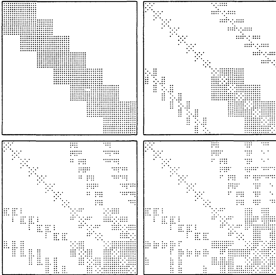
Figure 4.5: The matrices constructed in the transformation of I - T , matrices R_0, \dots, R_3 defined in Eq. (4.21), are shown for kernel K(x, t) = \log |x - t| , \epsilon = 10^{-3} , and n = 64 . The matrix R_4 looks like R_3 and is not shown.
