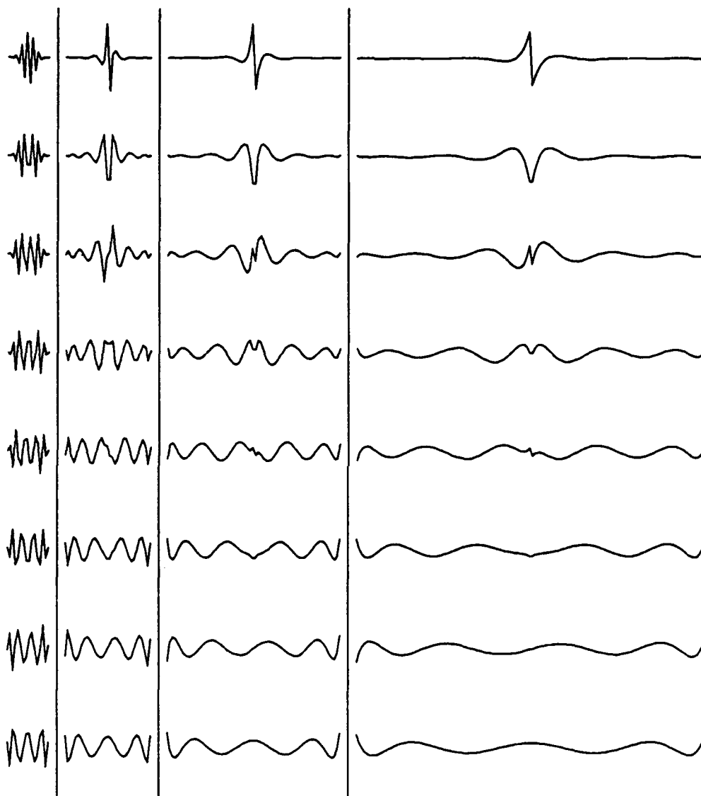
Figure 4.3: Basis vectors on four scales are shown for the basis where n = 128 , points x_1, \dots, x_n are equispaced, and k = 8 . The first column of vectors consists of rows 1–8 of U , the second column consists of rows 65–72, etc. Note that half of the vectors are odd and half are even functions, and that the odd ones are generally discontinuous at their center.
