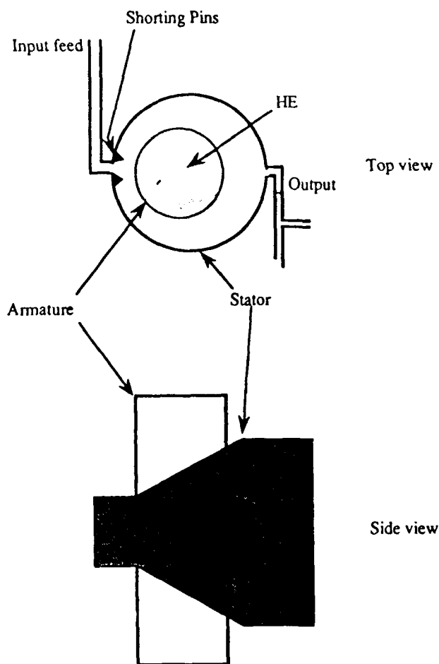
Figure 2. The M-10MJ, 10-MA Pavlovski Generator Described by Popkov
