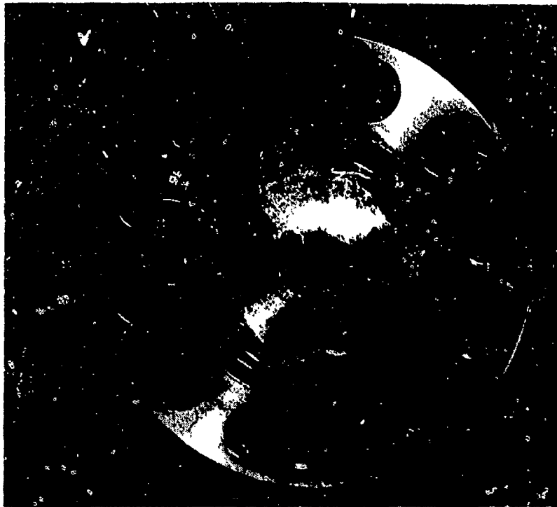
Fig. 4 — Confinement cell rear plate after explosion of HBX-1 sample, showing that most of the HE remained unreacted
