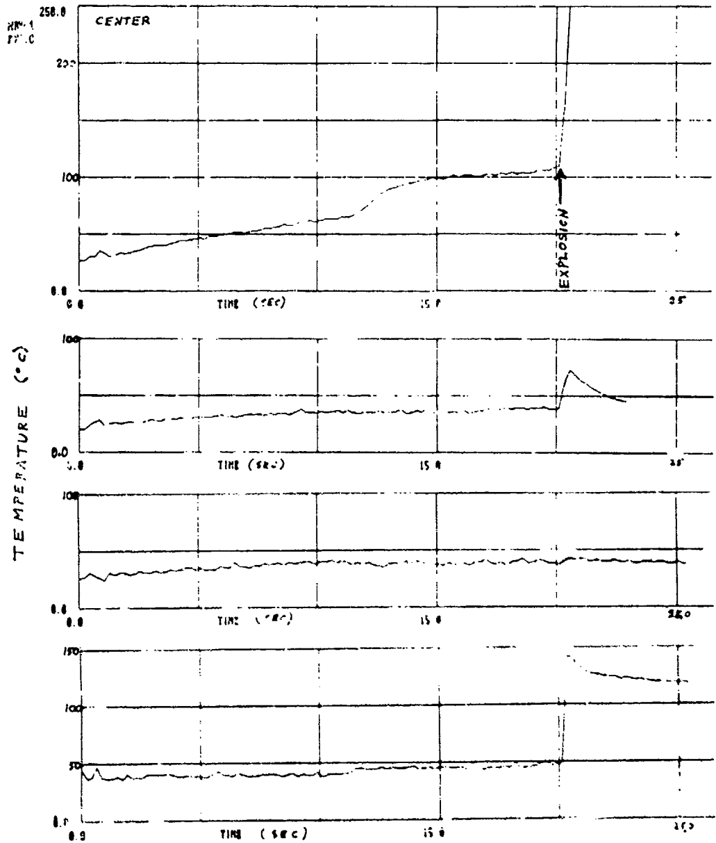
Fig. 5 — Thermocouple records for the center (top), and the three peripheral locations, showing that heat from the explosion of an HBX-1 sample spread anisotropically
