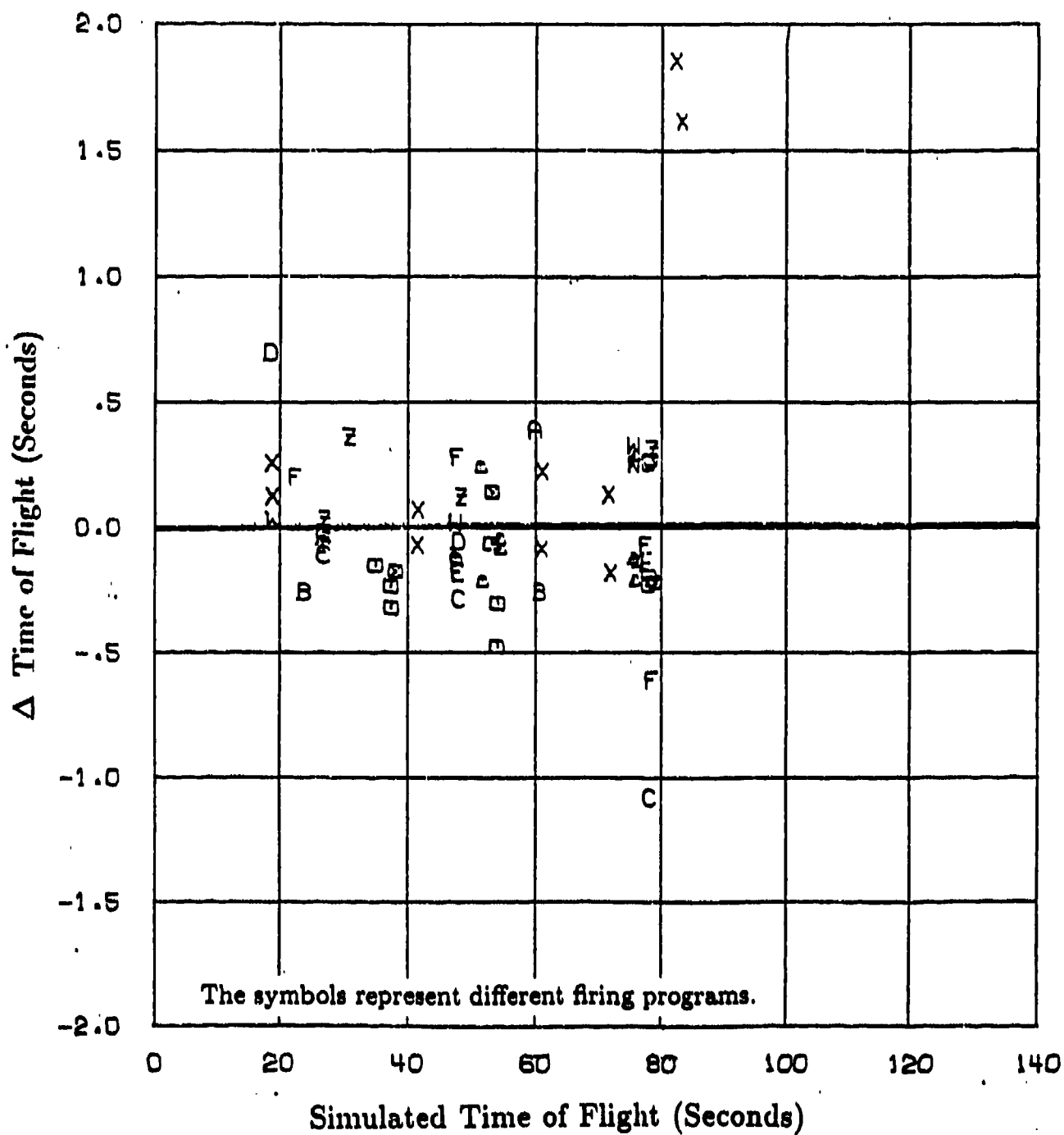
Figure 7. Difference between observed and simulated time of flight ( \Delta time of flight) versus simulated time of flight for projectile, 155mm, HE, M107 fired with propelling charge M4A2, charge 7W.
