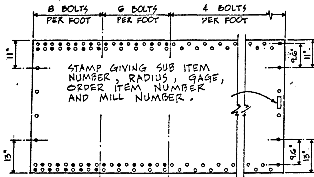
INSIDE VIEW
