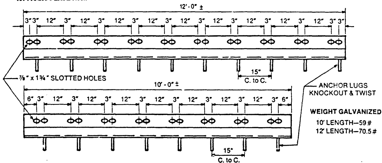
Figure 5. Unbalanced Channel for MULTI-PLATE Arch
