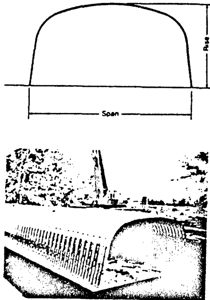
Figure 9. Box Culverts
