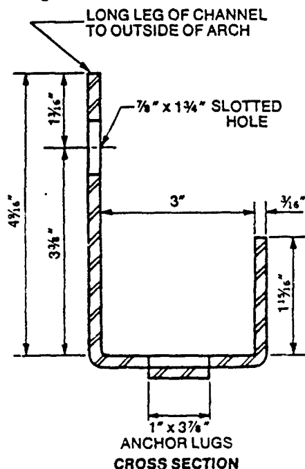
Figure 3. Channel Cross Section
