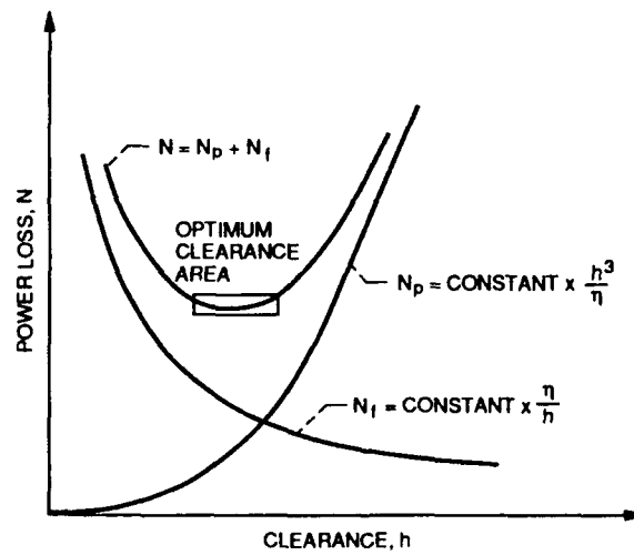
Figure 4. - Dependence of power losses on hydrostatic clearance.
