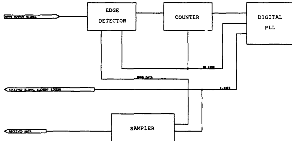
Fig. 5: Block Schematic of DATA Class 3 Clock Recovery Circuit
