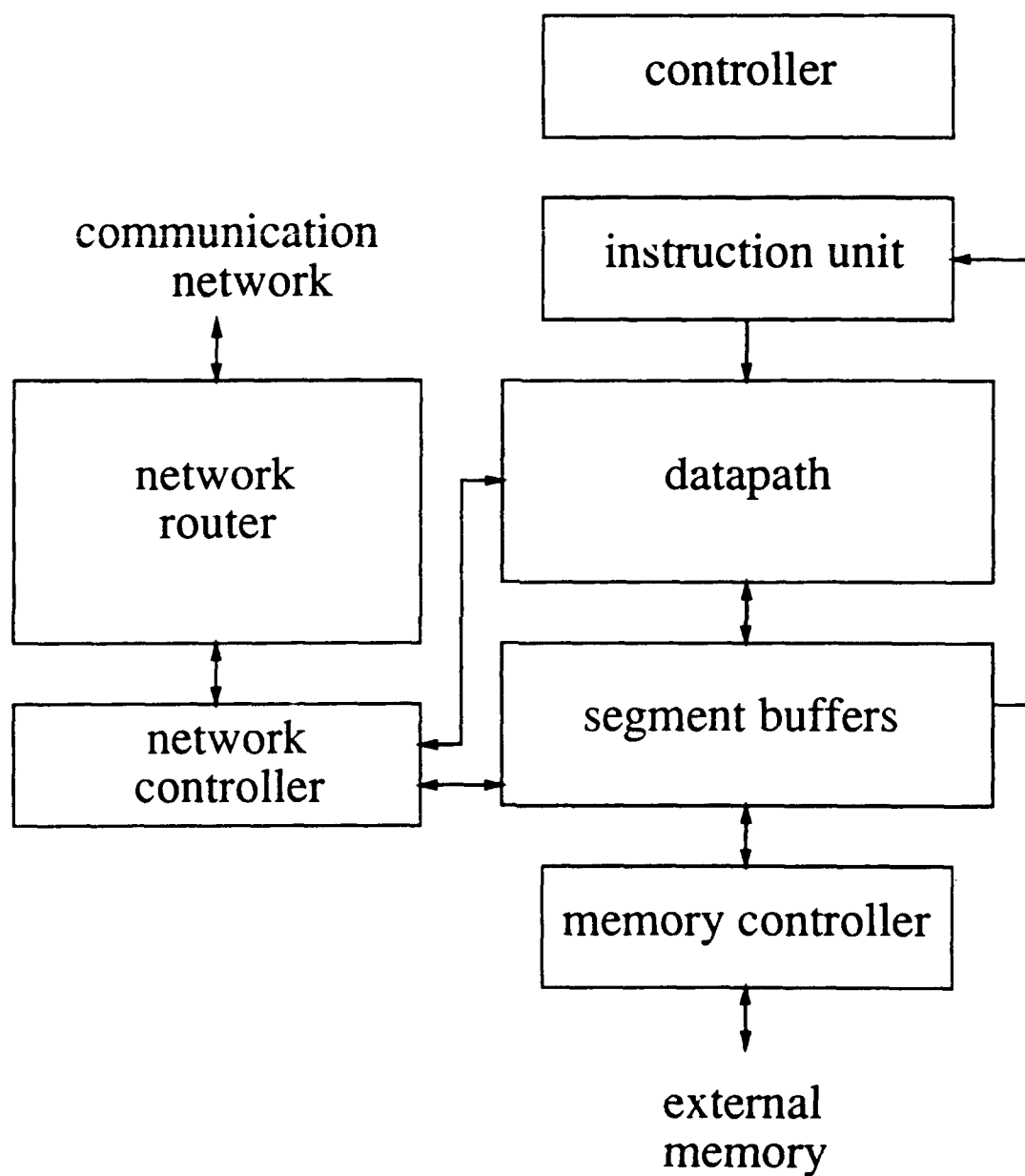
Figure 5.1: PiMac Microarchitecture
