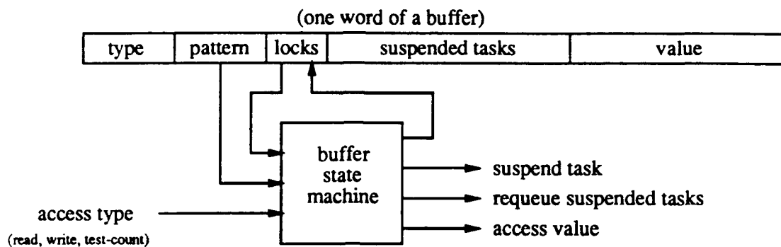
Figure 5.8: Buffer State Machine
