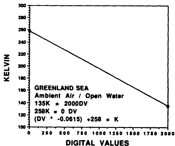
Figure A5. Brightness temperature conversion chart for 24 March 1987.
