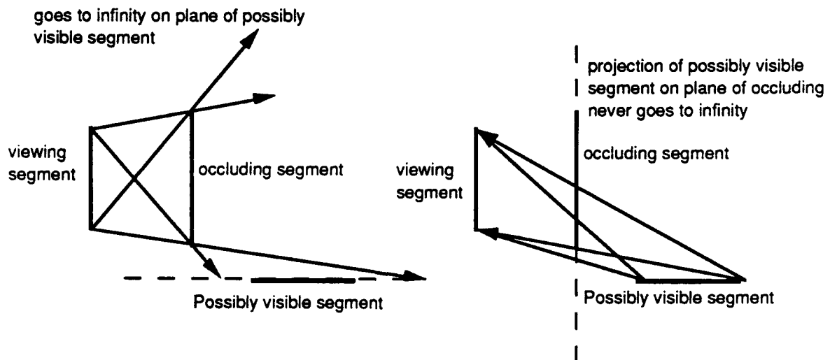
Figure 3.23 Projecting the possibly visible segment onto the plane of the occluding segment instead of projecting the occluding segment onto the plane of the possibly visible segment avoids the problem of projecting points to infinity.
