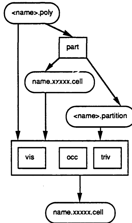
Figure 1.4. The programs used to compute the model subdivision or partition , and identify potentially visible sets. Vis computes the PVS for a cell with a sampling algorithm. Occ computes the PVS for a cell with an analytic algorithm. Triv simply assigns the polygons inside a cell to the PVS and is usually used only to evaluate the result of Partition .
