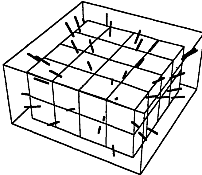
Figure 3.6 The jittered hemi-cube sampling pattern. Sample rays are shown extending through the sample areas. The sample rays start at the center of the base of the hemi-cube. This pattern transforms signal aliasing due to the coherence of the samples into (less objectionable) noise.
