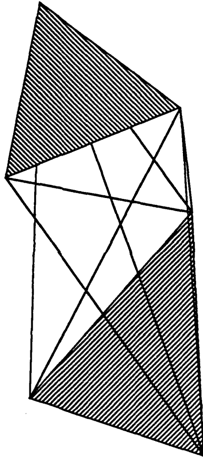
Figure 3.21 Define separators for two triangles embedded in 3D space by forming the planes defined by a vertex from one triangle and an edge from the other. Only some of these planes will qualify as separators. Each triangle must lie completely on opposite sides of the plane for it to qualify as a separator.
