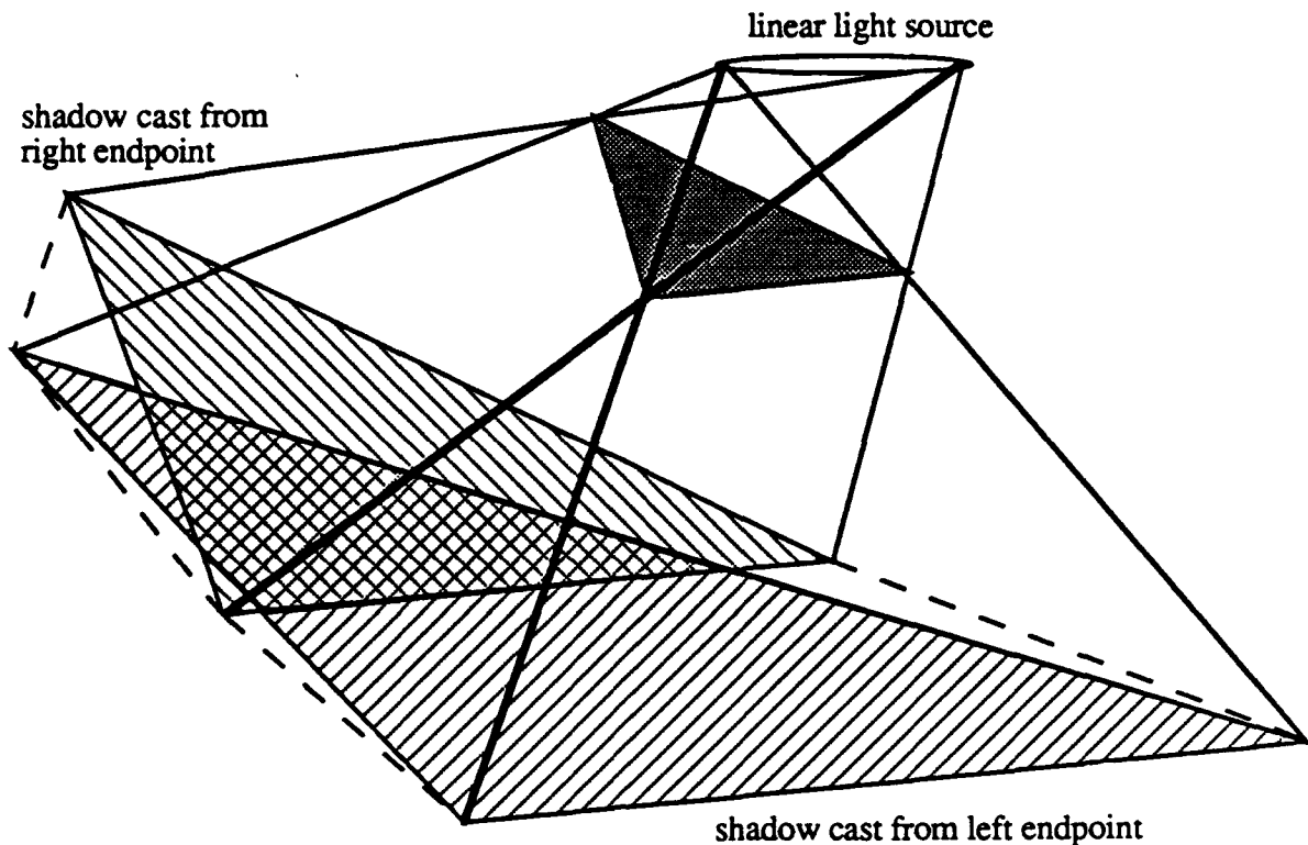
Figure 3.12 A Shadow Volume. The surfaces within the umbra receive no direct illumination from the area source. Surfaces within the penumbra but outside the umbra receive some fraction of the direct illumination of the linear source.
