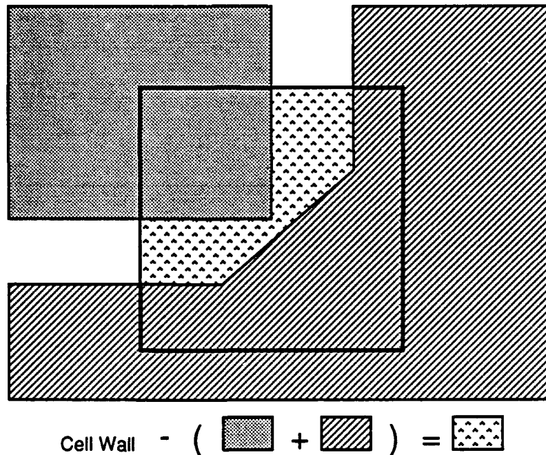
Figure 2.3 Portal computation. The rectangular cell wall is depicted by the bold rectangle. Polygons lying in the same plane as the cell wall are shown with thinner boundary lines. The portals are the set difference between the cell wall and the two polygons lying in the same plane as the cell wall.
