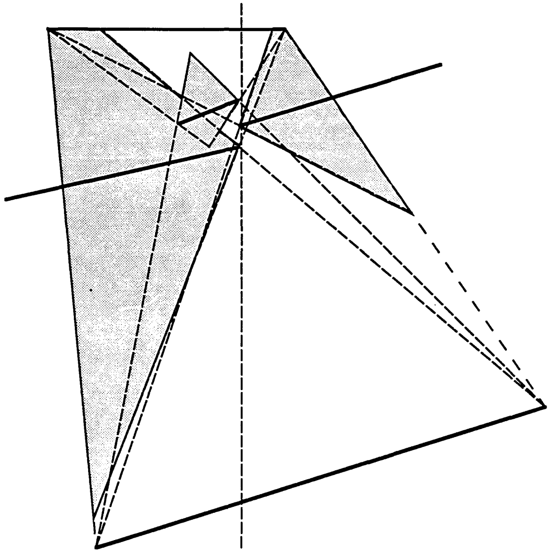
Figure 3.22 A counter-example to the idea of "cutting out the invisible portion between two polygons that might see each other". In this case, the dotted line represents the only way the polygon at the top can see the polygon at the bottom. The shaded area represents parts of the space between the two polygons that would be cut out by the effects of the occluding polygons. Moving any of the segments slightly to cut off the only line of sight does not separate the two polygons at top and bottom.
