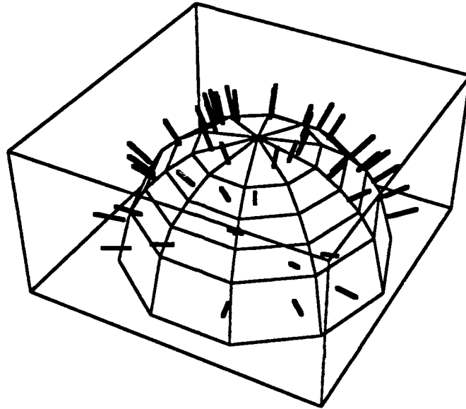
Figure 3.7 The angularly-jittered cosine-weighted-hemisphere sampling pattern. Sample rays are shown extending through the sample areas. The sample rays start at the center of the base of the hemisphere. This pattern has the property that each sample area has equal area when projected orthogonally down onto the base disk.
