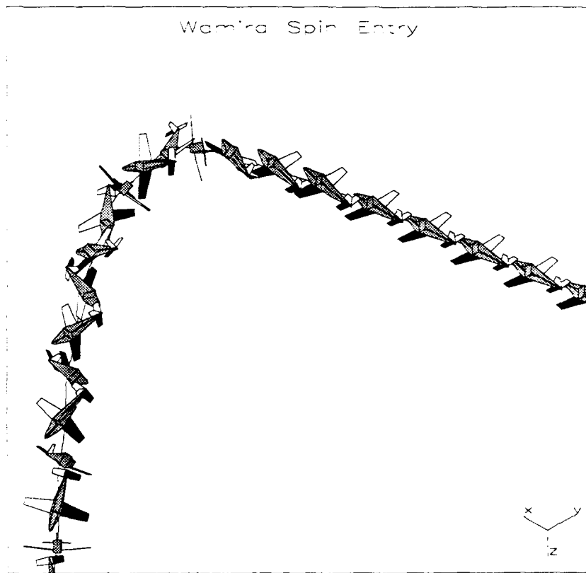
Figure 18. Three dimensional plot of aircraft spin entry.
