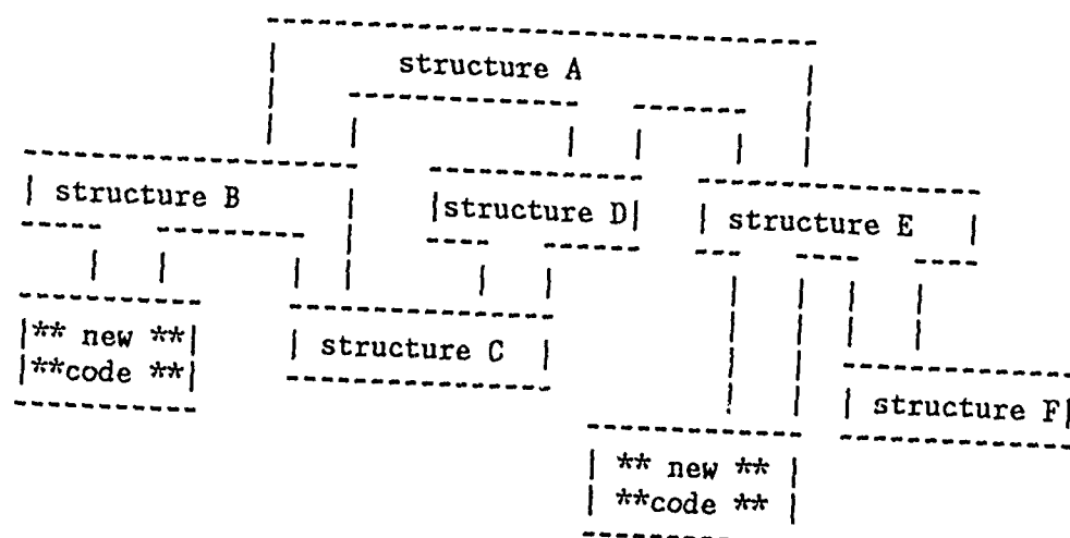
Figure 2. Compositional Reuse
