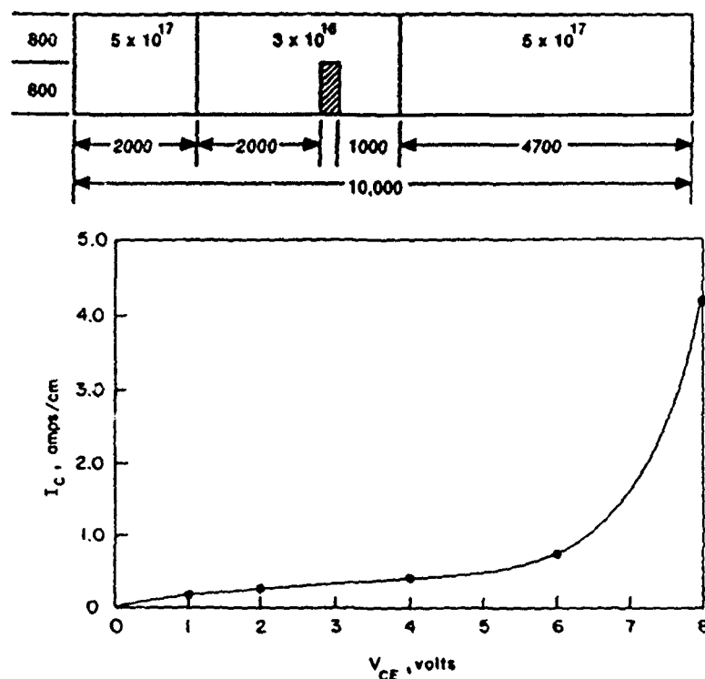
Figure 6. Structure and DC current-voltage characteristics of the PBT, structure B2, at a forward bias of 0.4v.
