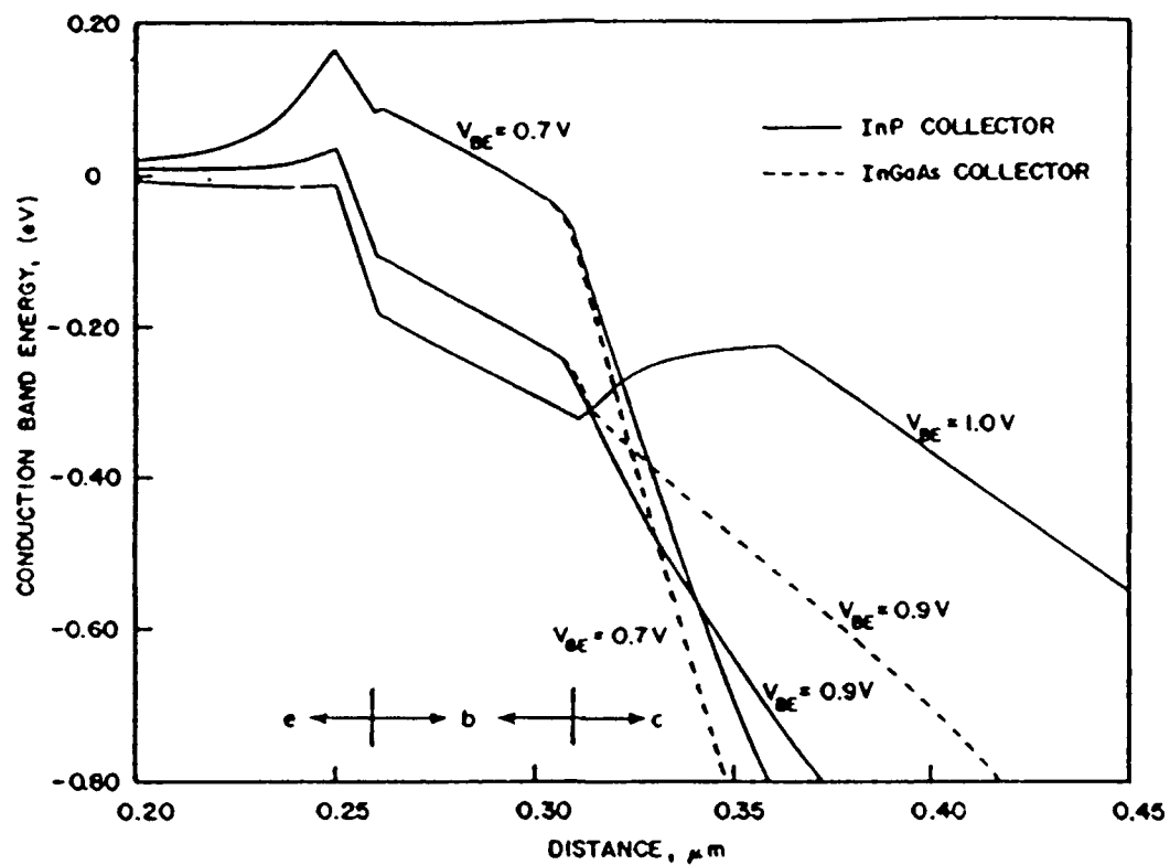
Figure 63. Conduction band diagram.
