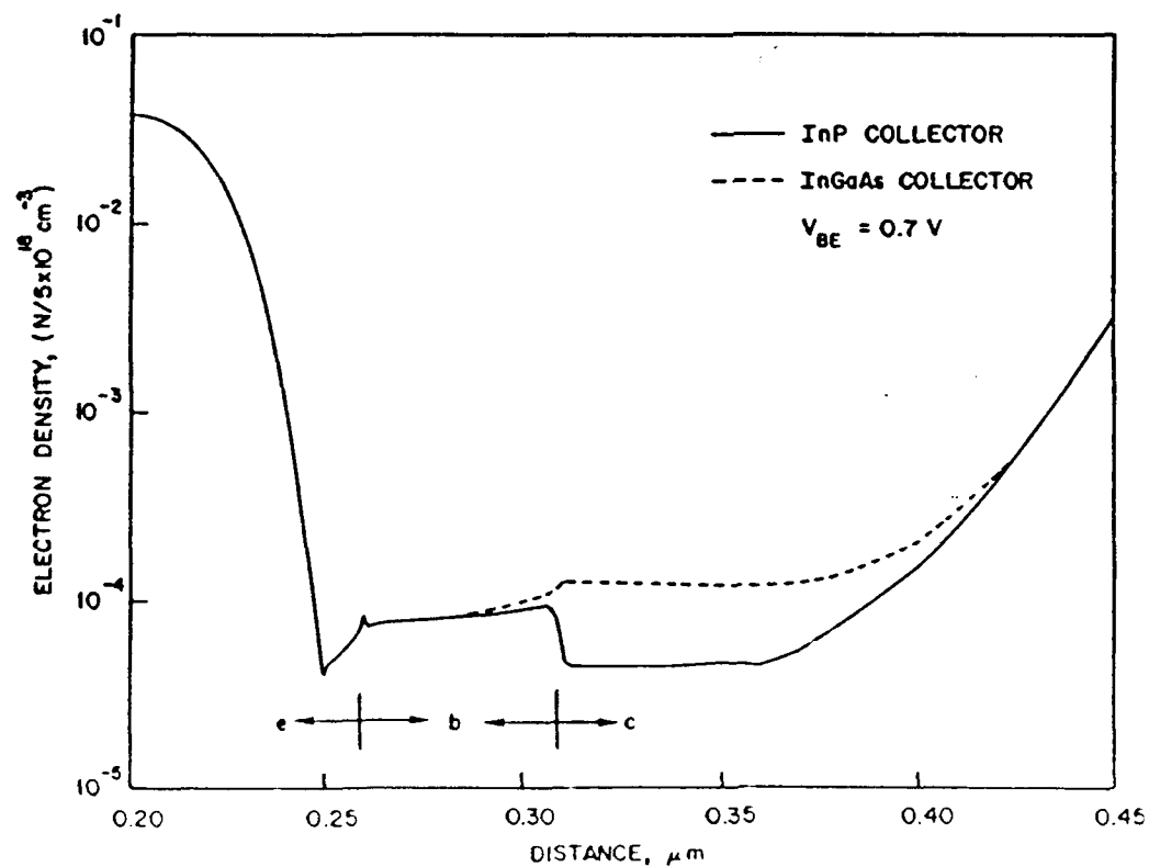
Figure 3. Electron Density Profile, V_{BE} = 0.7 v.
