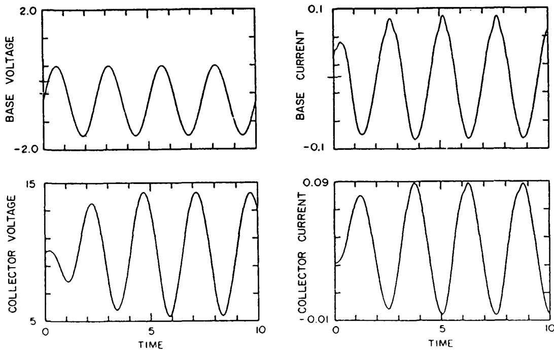
Figure 19. Time dependent current and voltage through the base and collector for V_b = -0.6 + 1.0\sin\omega t . The driving frequency is 40 GHz, f_r = 60\text{ GHz} , C = 5.10 \times 10^{-16} farads and L = 1.38 \times 10^{-8} henries.
