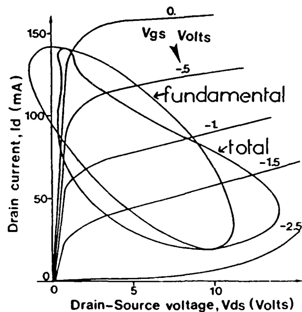
Figure 31. (a) Drain current-voltage lissajous for an input power of 15 mw a source-drain voltage of 3v, and a gate source voltage of -0.9v (these values are from ref (2)). (b) As in (a) but for a source-drain voltage of 5v.
