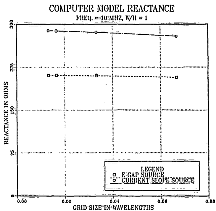
Figure 8. Comparison of voltage sources on resistance & reactance versus grid size for the W/H=1 antenna model.
