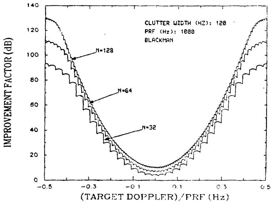
Figure 5: The Effect of Window Length (Blackman)
