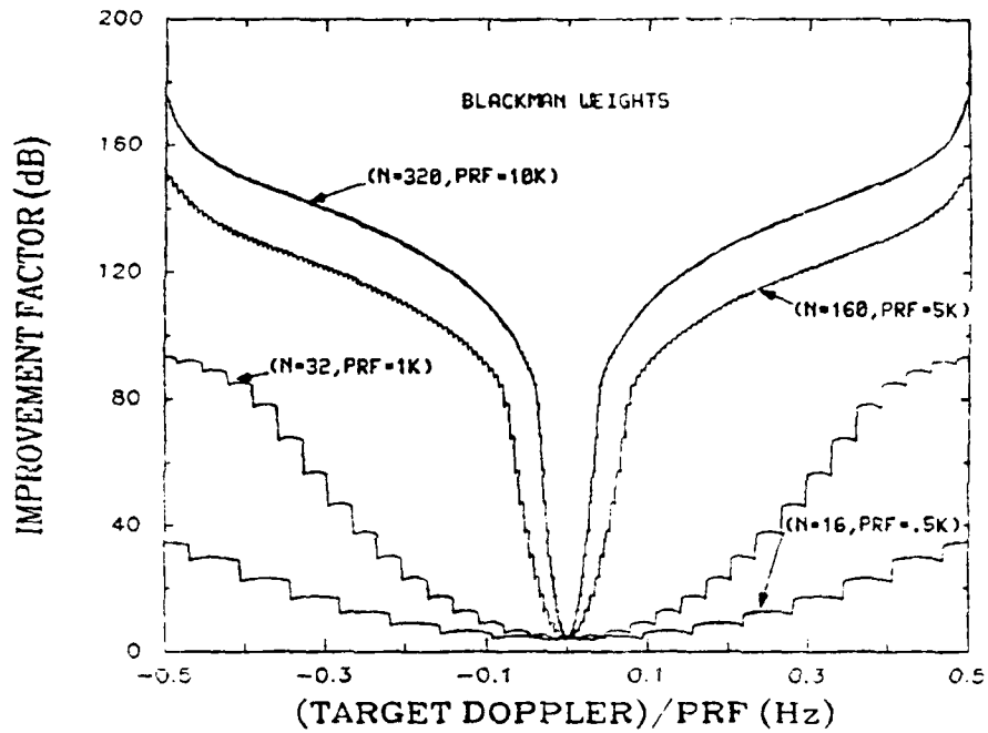
Figure 8 The Effect of the PRF (block size variable)
