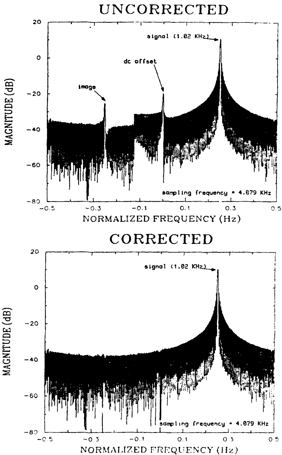
Figure 13 Example of Correction of I and Q for Doppler Frequency of 1.02 KHz
