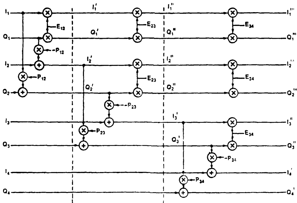
Figure 11 Multichannel Correction Process
