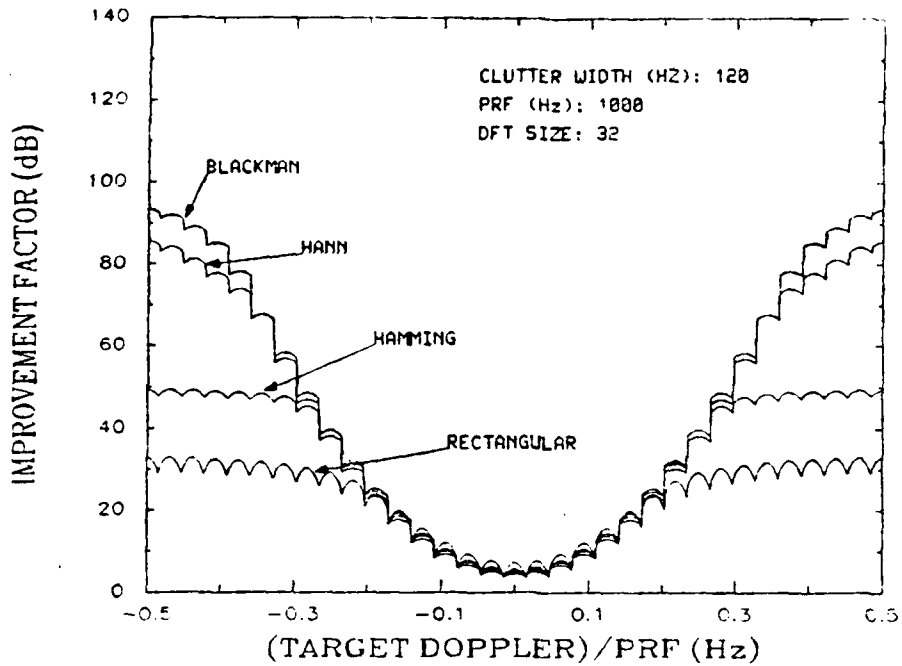
Figure 4: The Effect of Weighting Functions on the Improvement Factor
