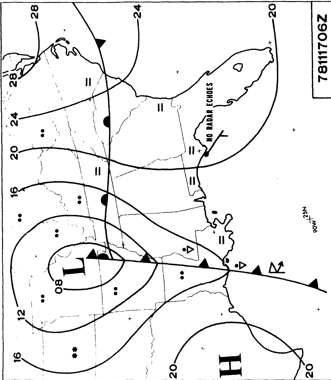
Figure 10-7 78111706Z Synoptic Chart
