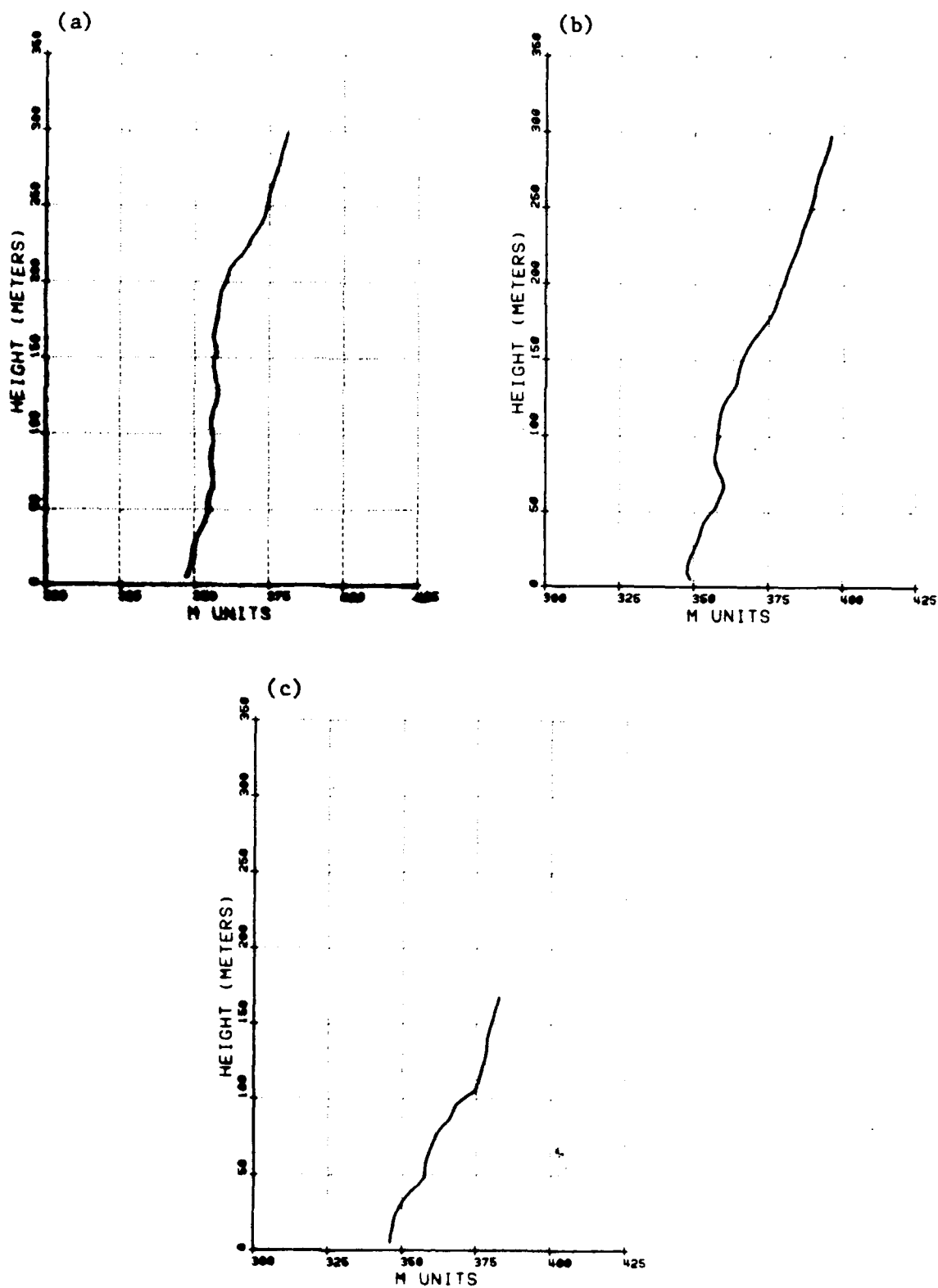
Figure 7-6 Case 7 M Profiles : a. Apalachicola, 22 Nov 78, 2200Z; b. Apalachicola, 23 Nov 78, 0900Z; c. Apalachicola, 23 Nov 78, 1000Z.
