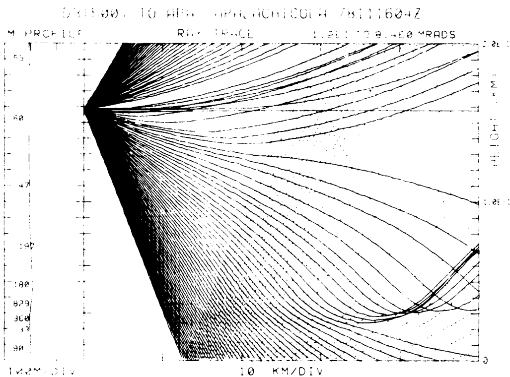
Figure 6-15. Case 6 Raytrace, D3(500) to APA, Apalachicola 16 Nov 78, 0400Z, Transmitter Height 158.4 m.
