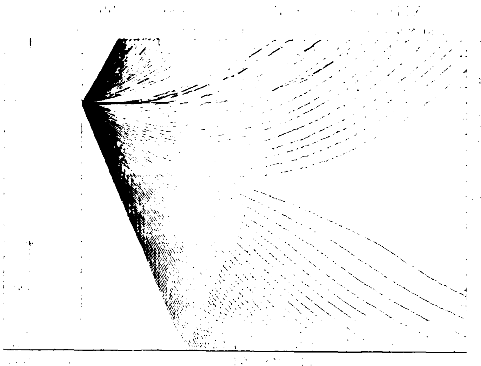
Figure 7-15. Case 7 Raytrace, D3(500) to APA, Cape San Blas 23 Nov 78, 1100Z, Transmitter Height 158.4 m.
