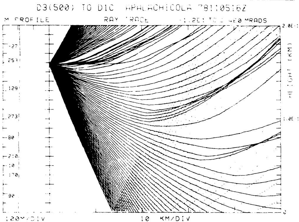
Figure 4-36. Case 4 Raytrace, D3(500) to D1C, Apalachicola 5 Nov 78, 1600Z, Transmitter Height 158.4 m.
