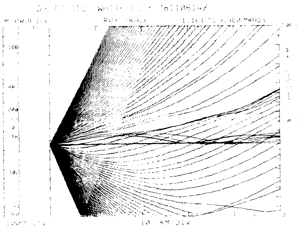
Figure 9-39. Case 9 Raytrace, D3 to D1C, White City, 6 Nov 78, 1400Z, Transmitter Height 76.2 m.
