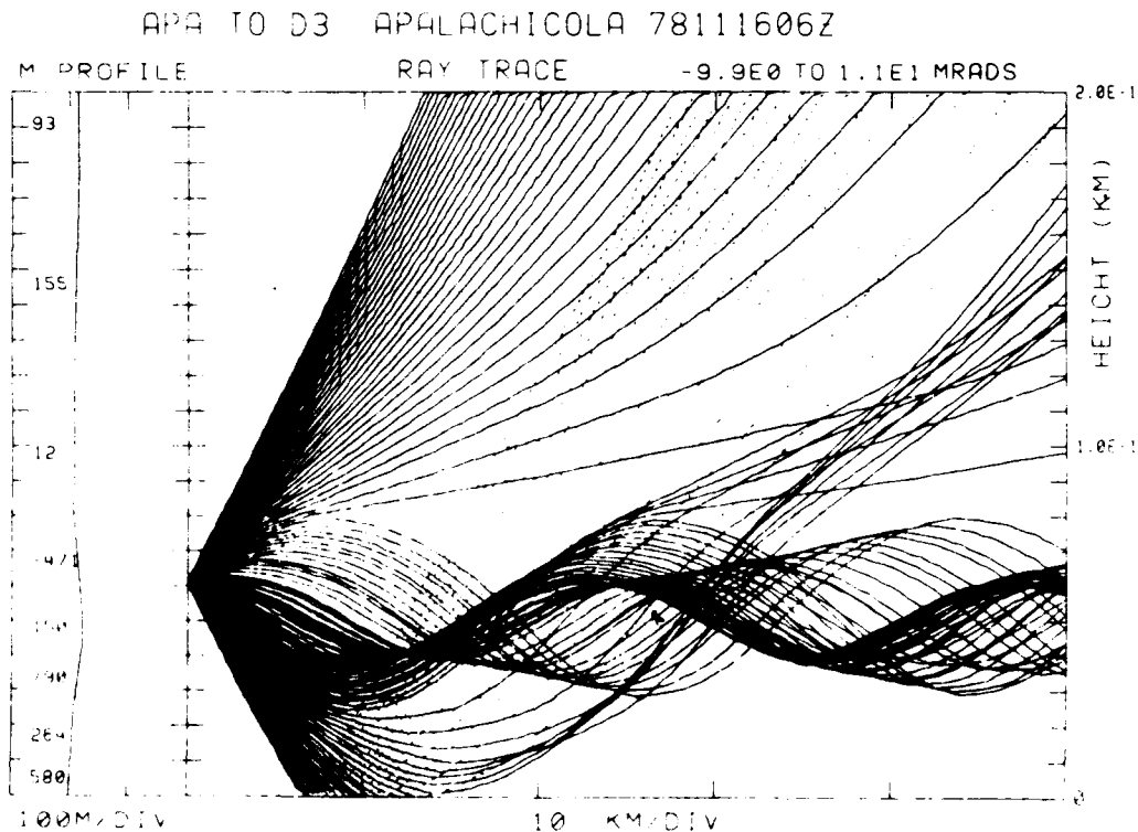
Figure 6-16. Case 6 Raytrace, APA to D3, Apalachicola, 16 Nov 78, 0600Z, Transmitter Height 61.0 m.
