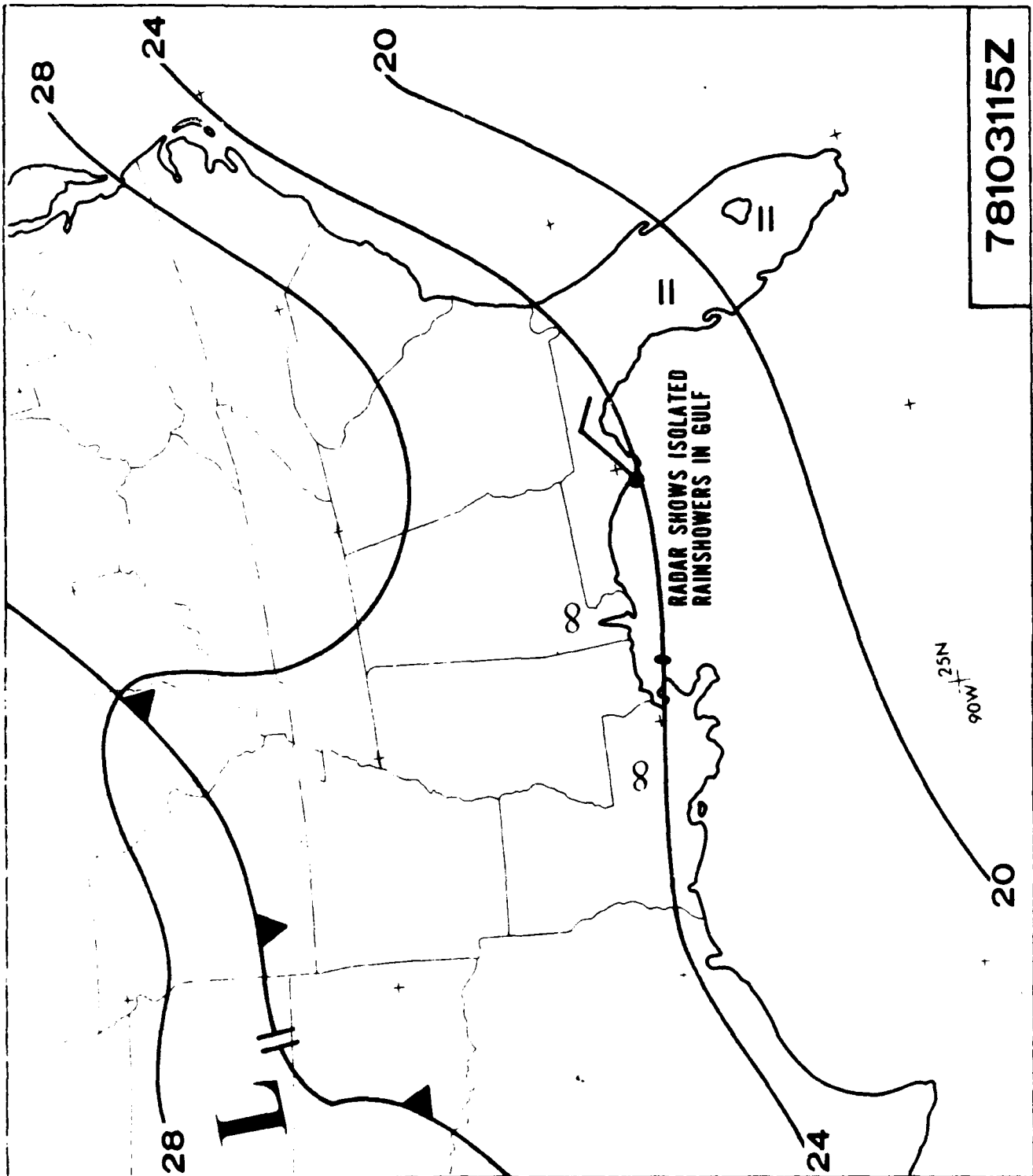
Figure 8-4 78103115Z Synoptic Chart
