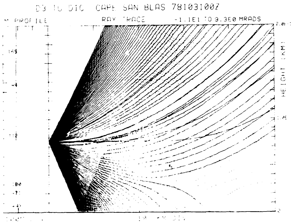
Figure 8-8. Case 8 Raytrace, D3 to D1C, Cape San Blas, 31 Oct 78, 0000Z, Transmitter Height 76.2 m.
