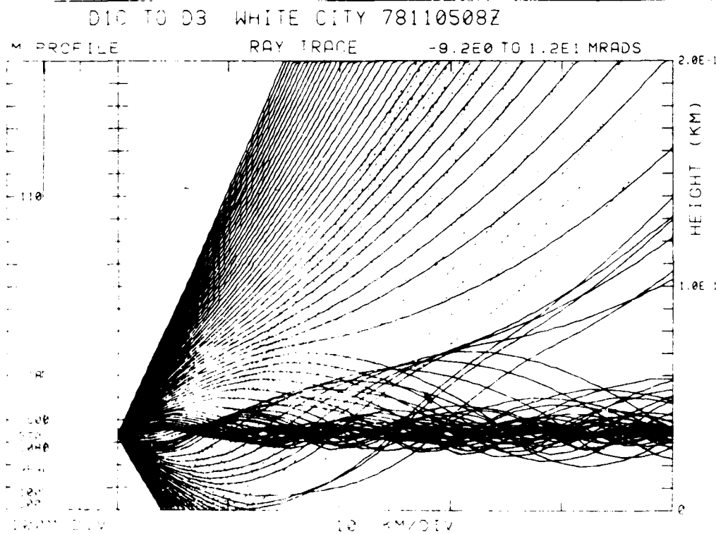
Figure 4-37. Case 4 Raytrace, D1C to D3, White City, 5 Nov 78, 0° Z, Transmitter Height 33.5 m.
