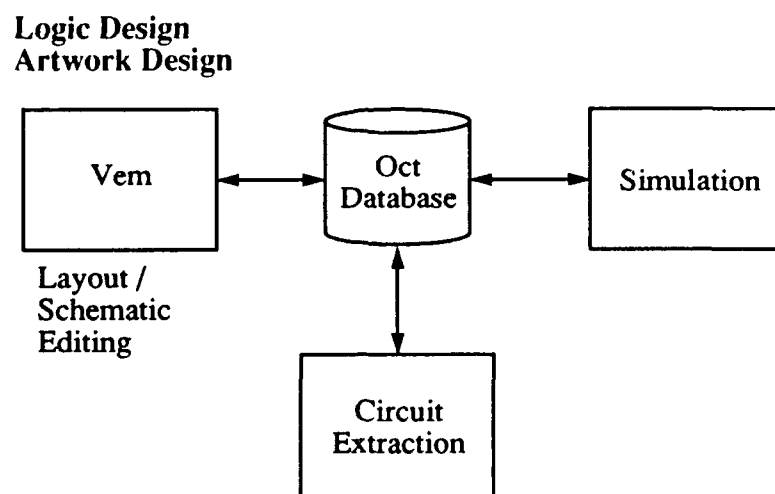
Figure 2.4b - An integrated design system using Oct/Vem
