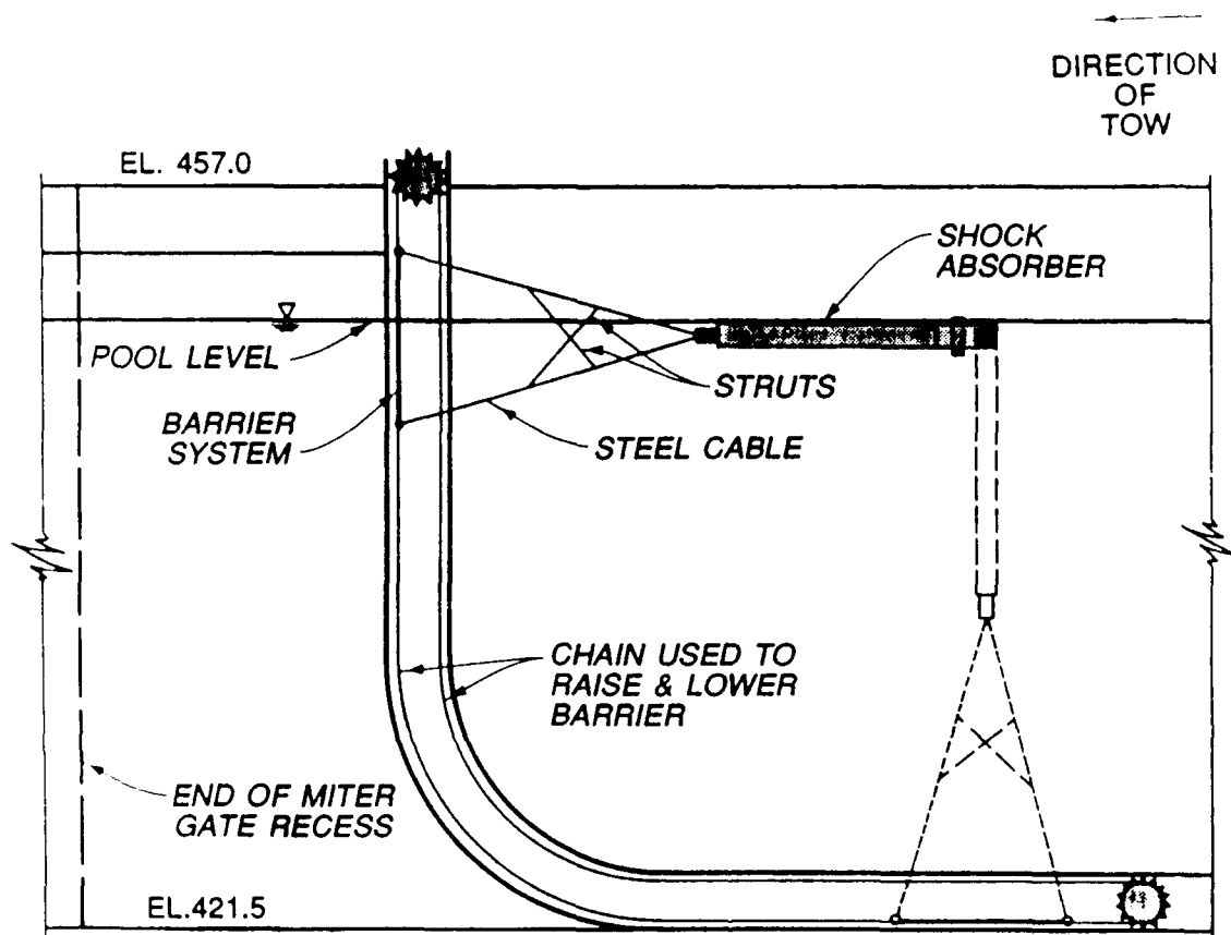
Figure A5. Side view of the raising and lowering mechanism
