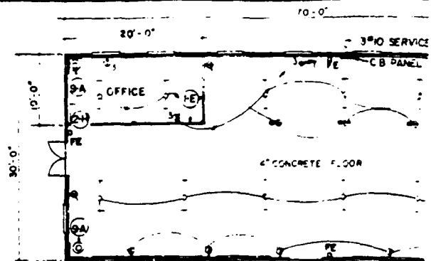
ADMINISTRATION - SUPPORT-BLDG. 30'x70'
