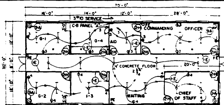
ADMINISTRATION - HEADQUARTERS-BLDG. 30'x70'
