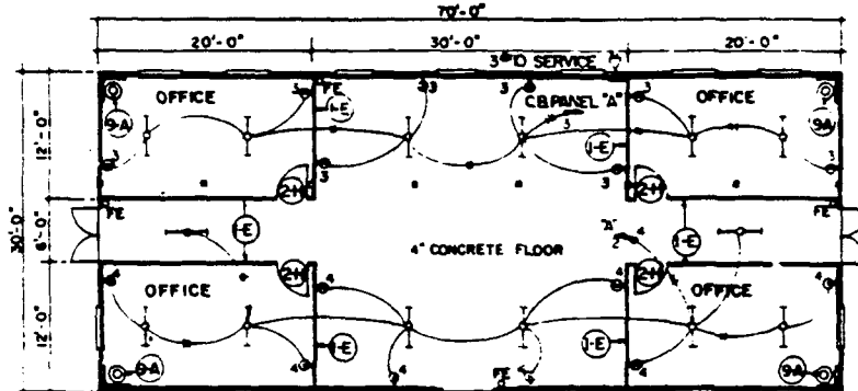
ADMINISTRATION - HEADQUARTERS-BLDG. 30'x70'
