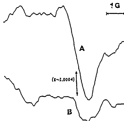
Figure 4 ESR traces of the \text{E}' center taken (A) after VUV illumination and (B) after subsequent ( hc/\lambda < 5.5 \text{ eV} ) UV illumination.
