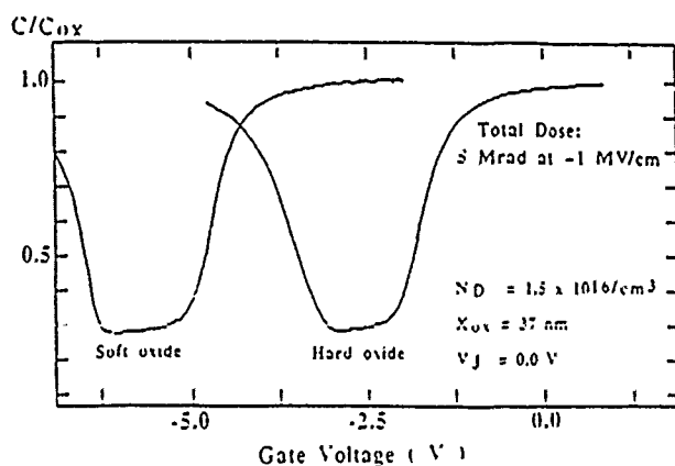
Figure 4 Post-irradiation HF CV curves for both hard and soft oxides.
