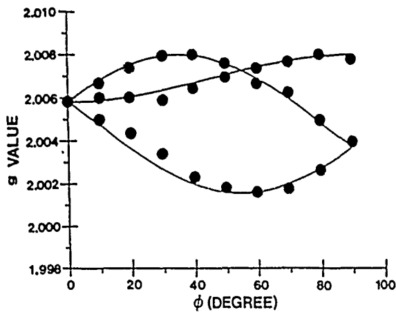
FIG. 4. ESR g -value anisotropy map for P_{b0} centers on (100) silicon substrates at different values of angle for rotation of the magnetic field in the (011) plane. The solid lines are given by the relation g^2 = g_1^2 \cos^2 \theta + g_2^2 \sin^2 \theta with g_1 = 2.0015 , g_2 = 2.008 , where \theta is the angle between the magnetic field and the [111] directions. The abscissa ( \phi ) in the figure is the angle between the magnetic field and the [100] direction.
