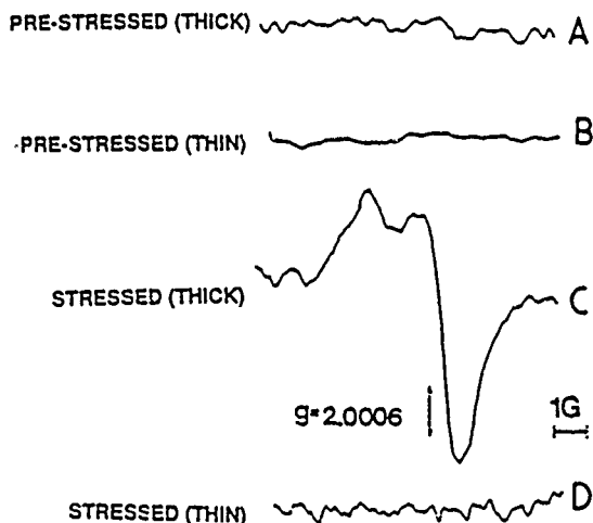
Figure 1: ESR Spectra. A and B - Spectra showing no paramagnetic centers for thick (A) and thin (B) oxides before stressing. C - Spectrum of an E' resonance after HFS a thick (1750A) oxide sample; D - Spectrum showing no E' resonance after HFS a thin (230A) oxide sample. (The magnetic field is parallel to the (111) plane of the Si/SiO 2 structure.)
