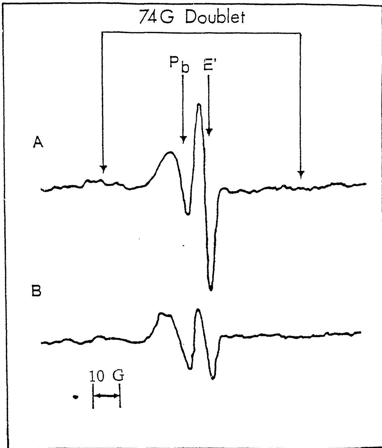
Figure 4. ESR resonances of an electron irradiated ( 20\text{keV} ) ( 10^{10}\text{ rad} ) \text{SiO}_2/\text{Si} structure (A) before anneal, and (B), after a 3 min 110^\circ\text{C} anneal in forming gas ( 5\%\text{H}_2/95\%\text{N}_2 ). Following the anneal, \text{E}' decreases significantly, but no 74G doublet resonance is detected. Spectrometer settings for both traces are identical, and are set to maximize the 74 G doublet resonance amplitude.
