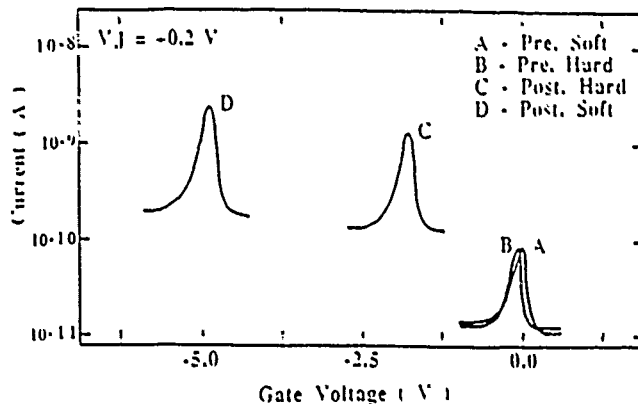
Figure 3 Pre- and post-irradiation IV curves for both hard and soft oxides.
