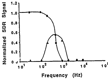
Fig. 9. P_{b0} center's in-phase and out-of-phase SDR signals versus magnetic field modulation frequency.
