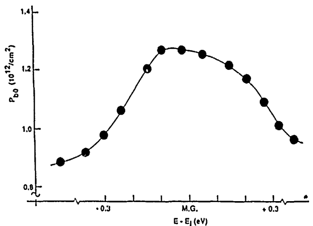
FIG. 6. Population of paramagnetic P_{b0} centers vs Fermi level. Results were obtained from the data of Fig. 5.
