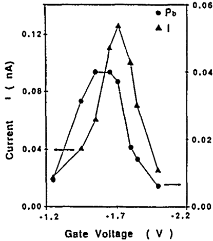
Fig. 7. (left) Recombination current ( I ) and P_{b0} center SDR signal ( \Delta I ) versus gate voltage for the hard device.
