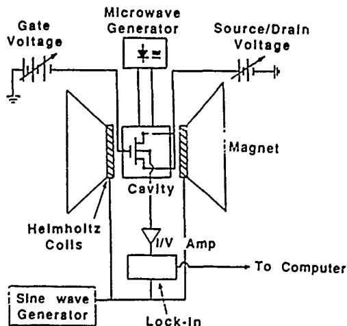
Fig.3. Block diagram of the SDR spectrometer.
