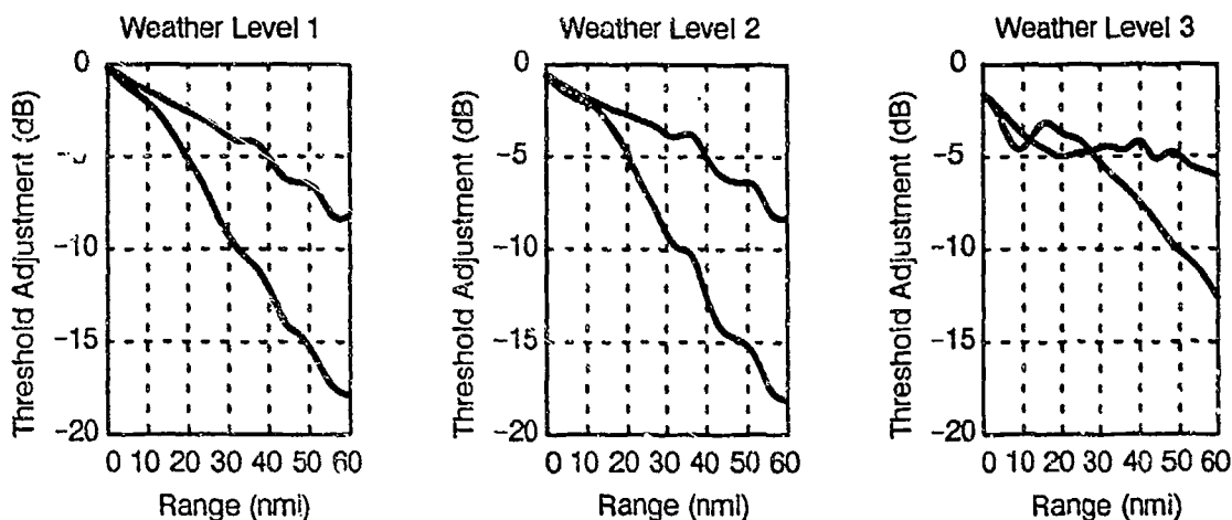
Figure 20. Threshold adjustments as in Figure 16, but for the Seattle data set.
