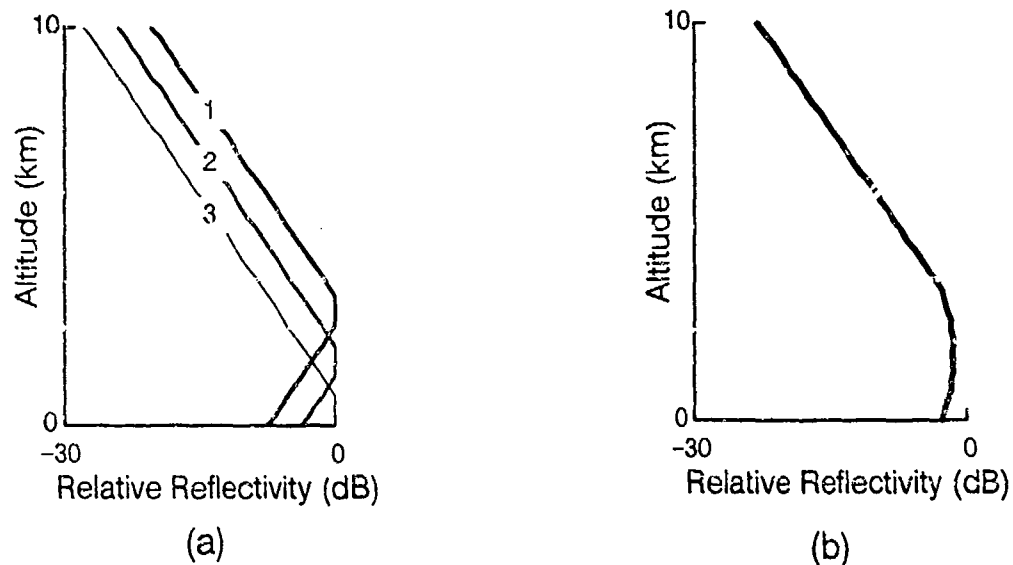
Figure 6. Illustration of vertical reflectivity profile averaging process: (a) Superimposed set of normalized profiles, (b) Mean profile derived from averaging of normalized profiles.
