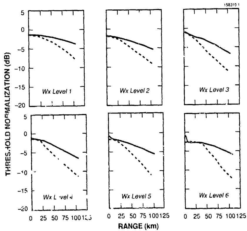
Figure 8. ASR-9 6-level weather threshold normalizations for New England convective storms. Solid and dashed curves are low and high beam adjustments, respectively. (From Weber, 1986.)
