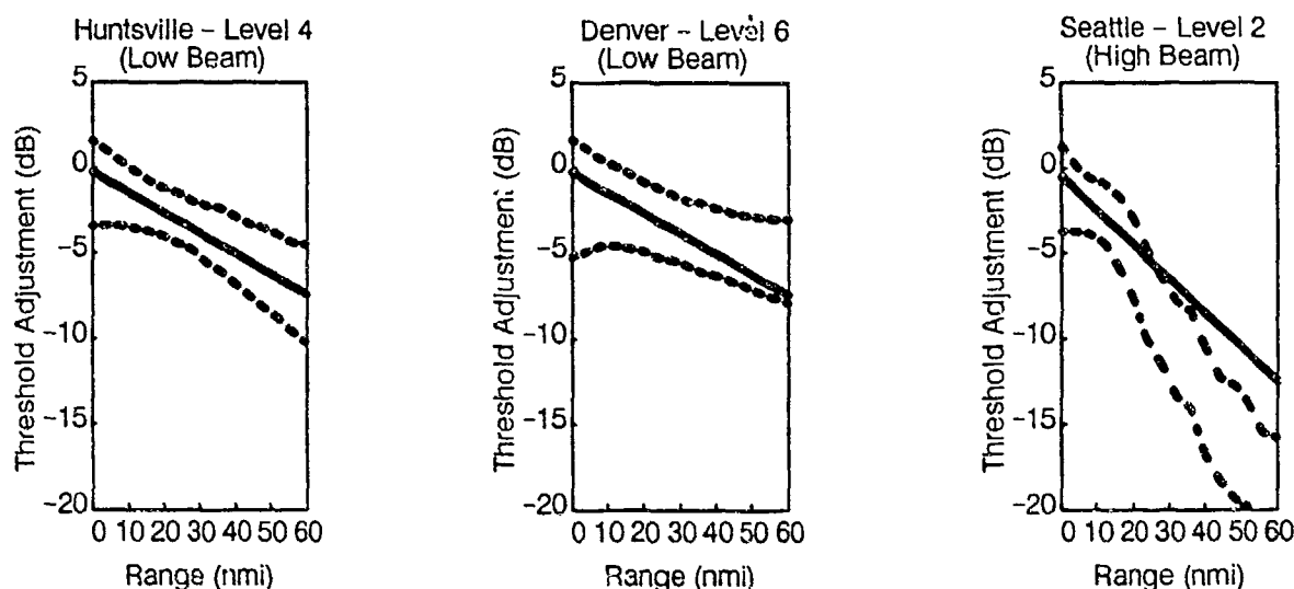
Figure 21. Relative placement of U.S. threshold adjustment curve (solid) with respect to upper and lower rms error bounds of site/level specific adjustment curves (dashed).
