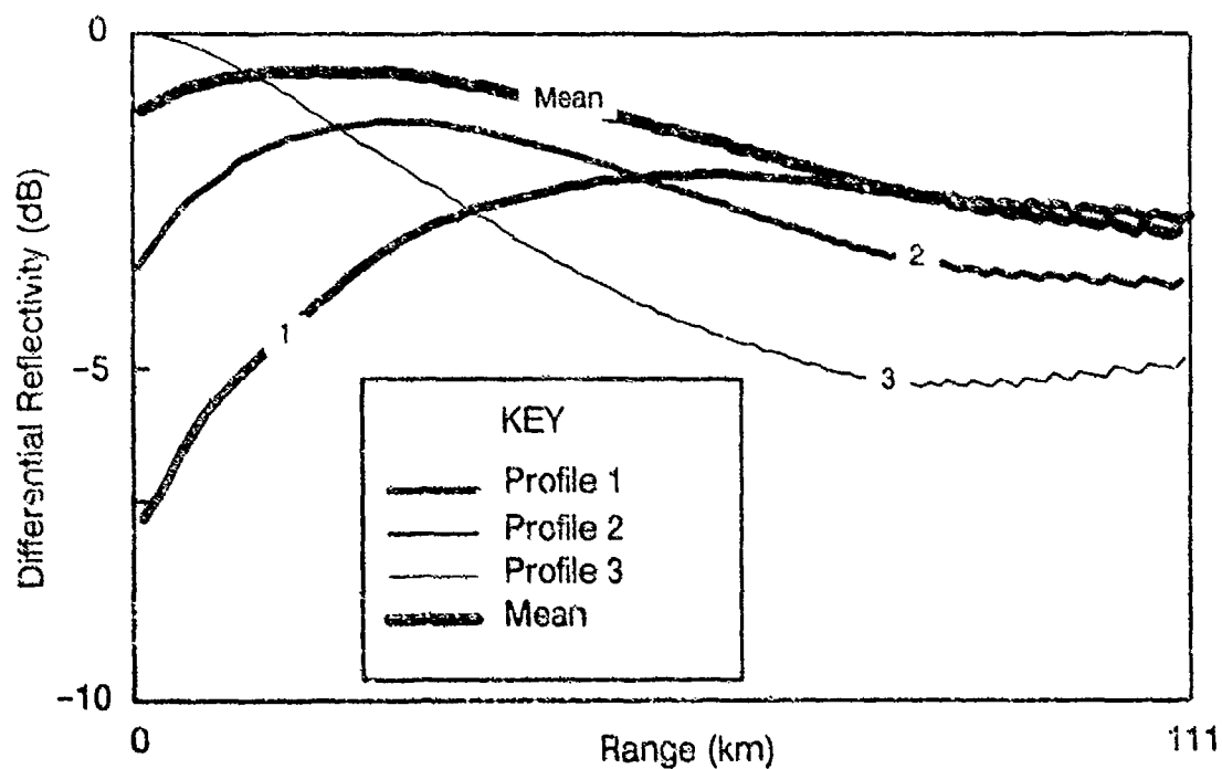
Figure 7. Reflectivity difference between the uncorrected ASR-9 reflectivity (low beam) and the vertical profile maximum for the three profiles and their mean shown in Figure 6.
