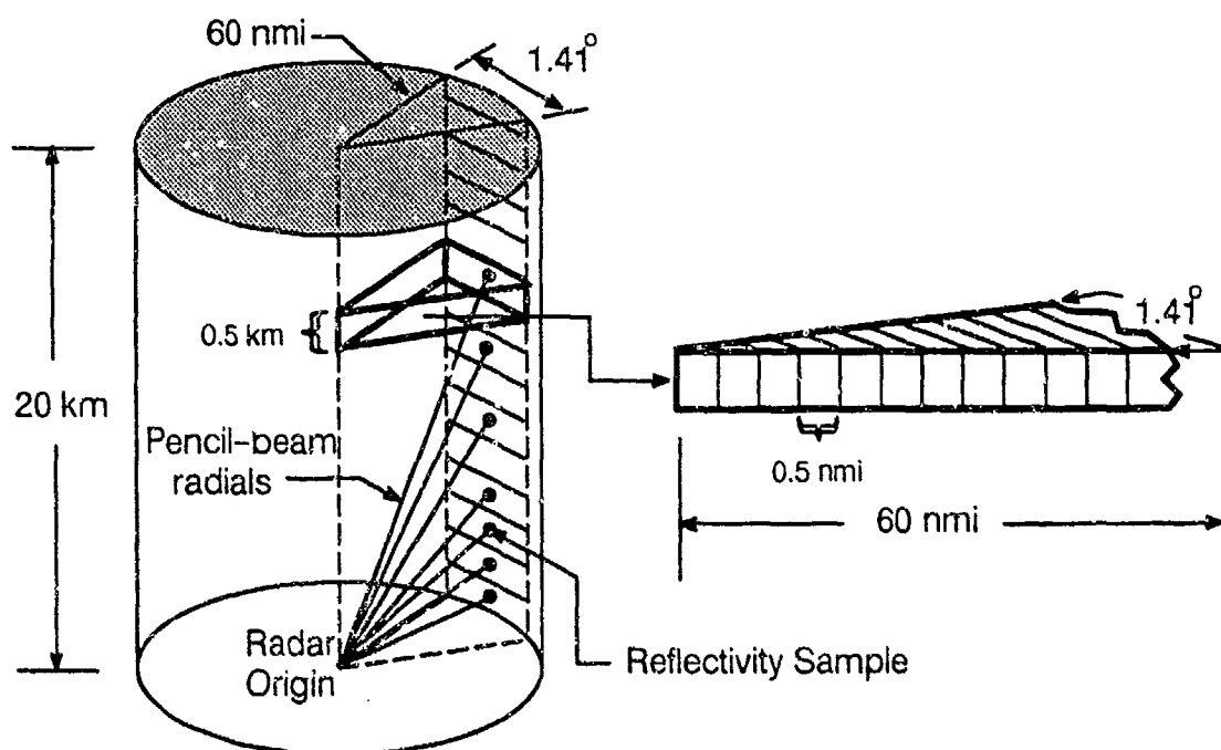
Figure 12. Schematic depiction of profile cylinder geometry.
