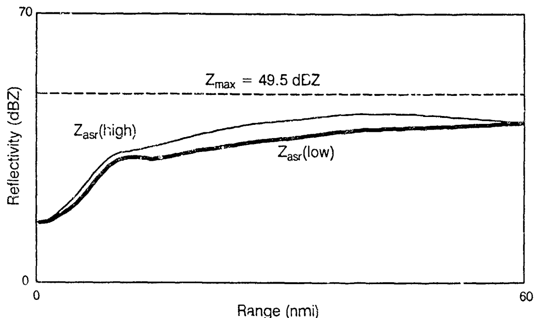
Figure 15. Z_{max} and Z_{asr} (low and high beams) computed from reflectivity profile of Figure 14. An ASR antenna tilt of 2.0^\circ was assumed for computation of Z_{asr} .
