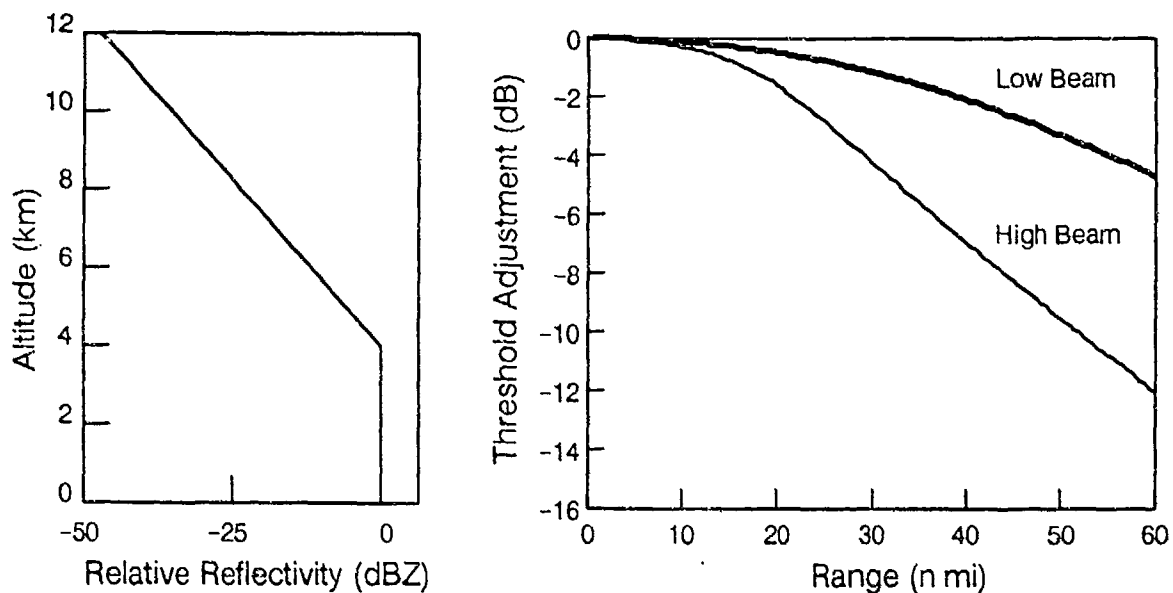
Figure 10. Current ASR-9 reflectivity profile model (left) and corresponding threshold adjustments (right).
