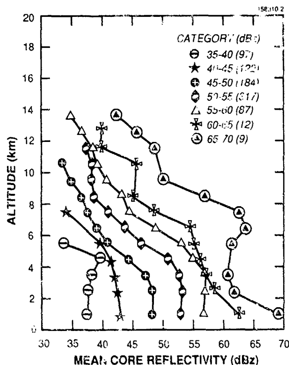
Figure 5 Profiles of mean core reflectivity for various categories of rainshowers. Number of cells in each category is shown in parentheses. (From Konrad, 1978.)
