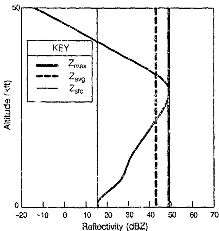
Figure 14. Vertical reflectivity profile through Denver thunderstorm on July 3, 1987 at azimuth 162.0°, range 26.5 nmi. Vertical lines indicate Z_{\max} , Z_{\text{avg}} , and Z_{\text{sfc}} for the profile shown (see key).
