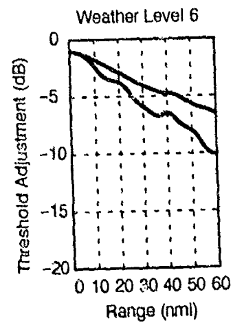
Figure 18. Threshold adjustments as in Figure 16, but for the Kansas City data set.
