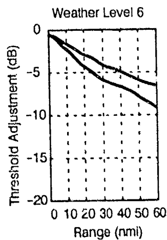
Figure 16. Threshold adjustments necessary to minimize the report error of the ensemble of profiles comprising each weather level in the Boston data set. Upper curve is for the low beam, lower curve for the high beam.
