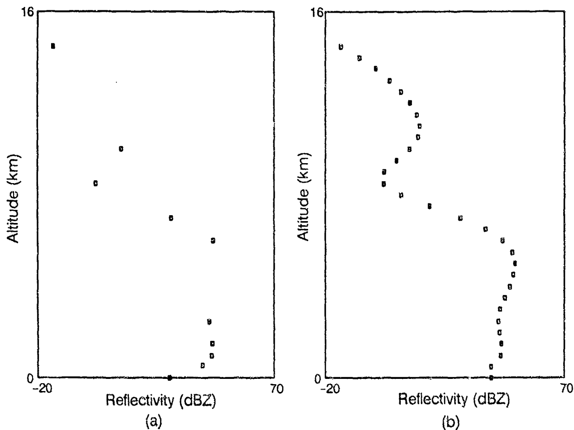
Figure 13. Vertical reflectivity profile (a) before and (b) after filtering and filling.
