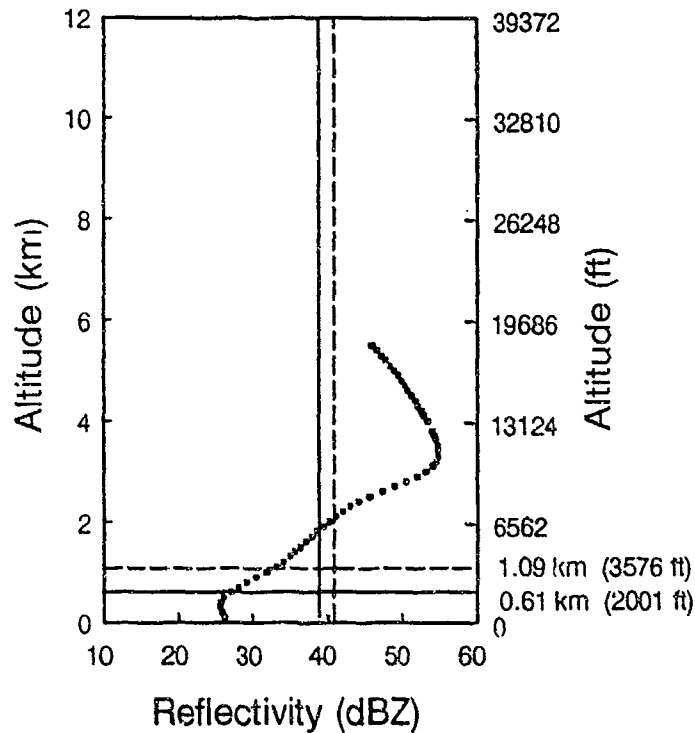
Figure 24. Example reflectivity profile where Z_{max} is at least two weather levels greater than the corrected Z_{asr} (low beam Z_{asr} is shown with solid vertical line, high beam Z_{asr} is shown with dashed vertical line). Altitude extents of the upper 3 dB edge of the high and low beam are indicated with dashed and solid horizontal lines respectively. The profile is from Denver taken on 9/5/87 at approximately 23:20 UTC and was located at 61^\circ azimuth, 4.3 nmi range.
