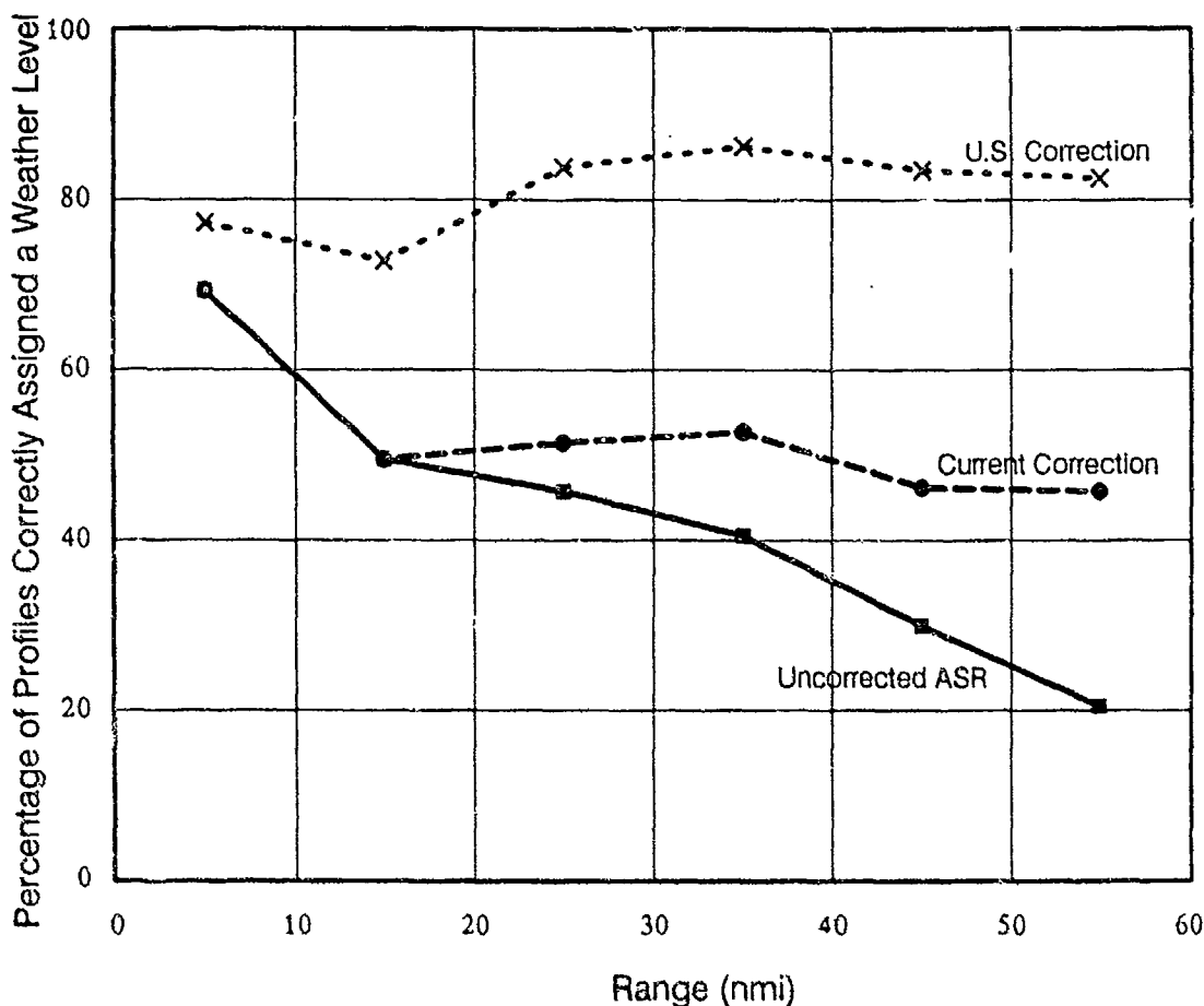
Figure 22. Percentage of cells in weather levels 2 through 6 for all sites that are correctly quantized. Solid line with filled boxes represents uncorrected quantization of ASR reported reflectivity. Dashed line with circles represents quantizations adjusted with current correction. Dotted line with x's represents quantizations adjusted with a single U.S. correction for all sites and weather levels.
