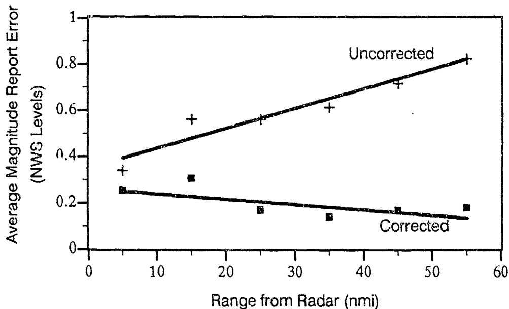
Figure 23. Average weather report error versus profile range from radar for the entire test data set. Errors without any correction (upper line, plusses) clearly exceed errors after correction (lower line, filled squares).
