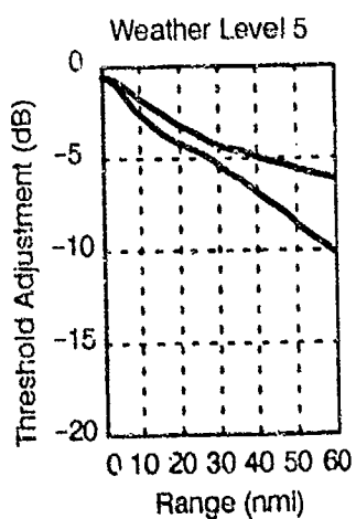
Figure 16. Threshold adjustments necessary to minimize the report error of the ensemble of profiles comprising each weather level in the Boston data set. Upper curve is for the low beam, lower curve for the high beam.
