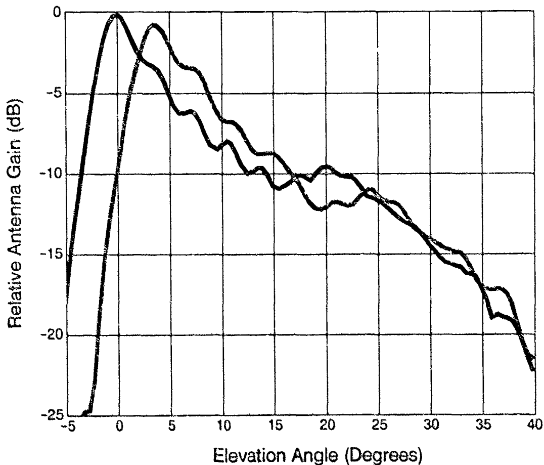
Figure 1. ASR-9 antenna pattern in the principal elevation plane. The low beam is plotted with a black curve and the high beam is plotted with a gray curve. The antenna is assumed to be positioned parallel to the horizon.
