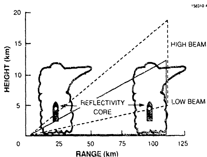
Figure 3. Schematic illustration of ASR-9 beam filling problem. Altitude limits of the -3 dB points on the ASR-9 antenna pattern are shown for the high (dashed) and low (solid) beam. A 2.0^\circ antenna tilt is assumed.
