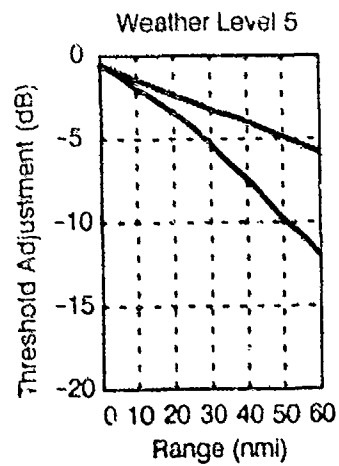
Figure 17. Threshold adjustments as in Figure 16, but for the Huntsville data set.
