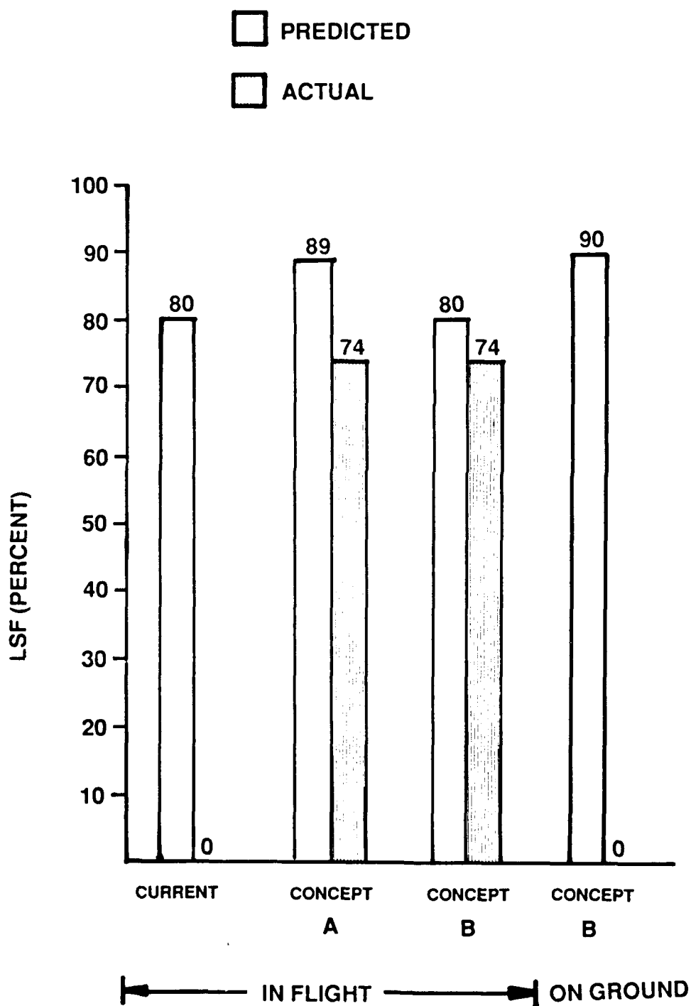
FIGURE 10. PREDICTED VERSUS ACTUAL LSF FOR FORWARD SMOKE GENERATION
