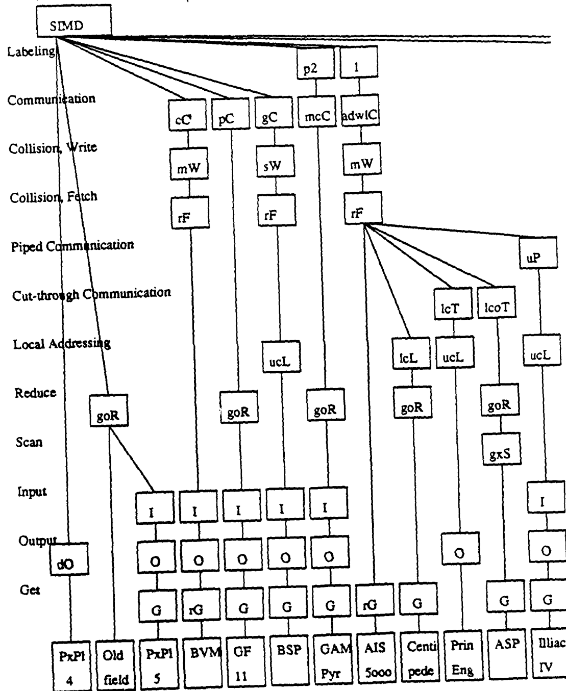
Figure 3.3: Tree of SIMD Architecture Classifications. The remainder of the tree is shown in the next figure.
