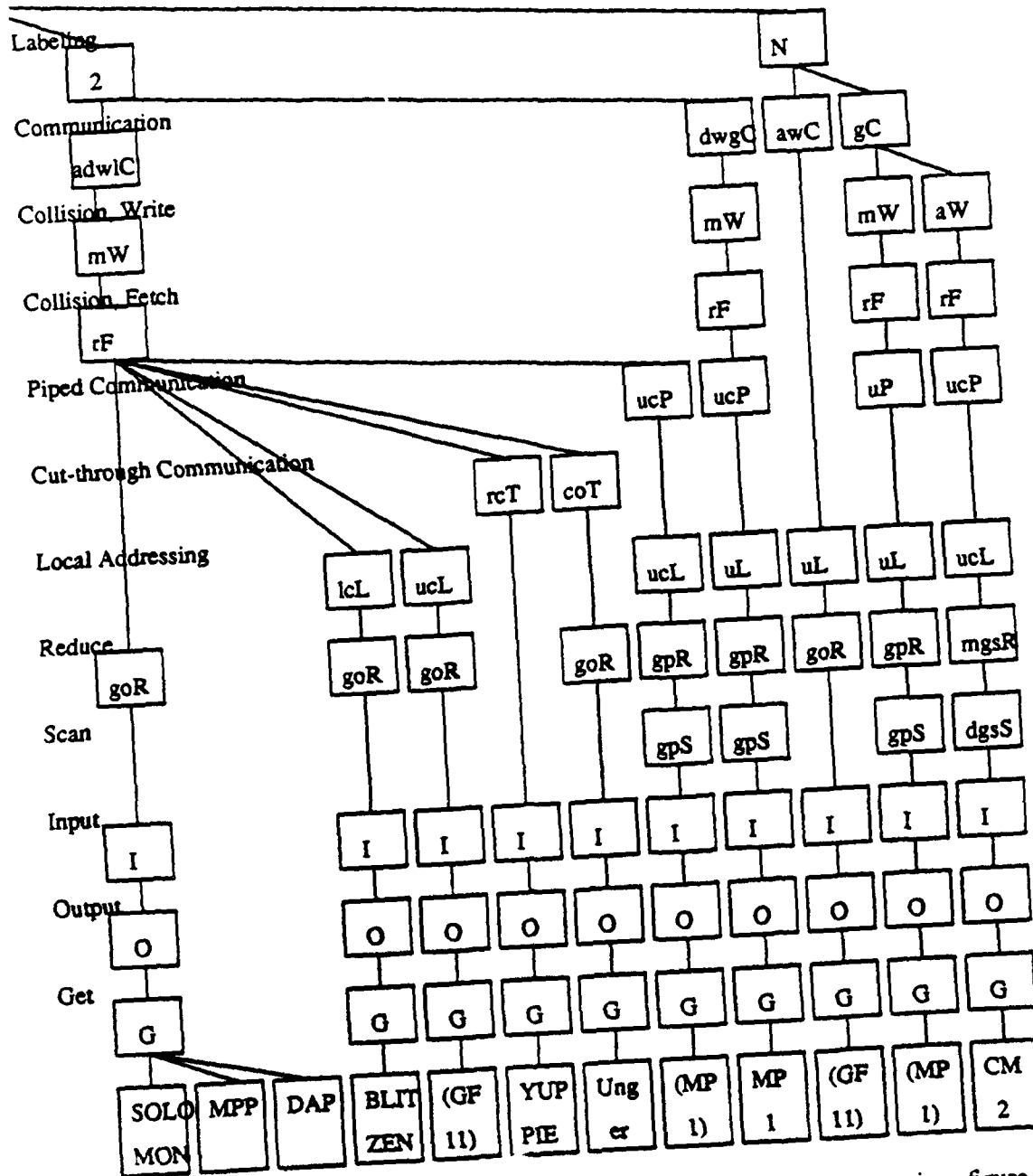
Figure 3.4: Tree of SIMD Architecture Classifications, continued from the previous figure.
