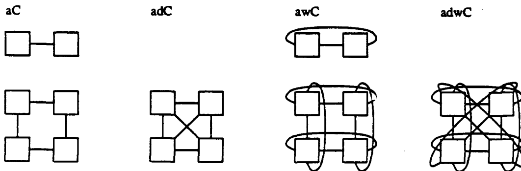
Figure 3.1: 1-D and 2-D Adjacent Communication Networks
