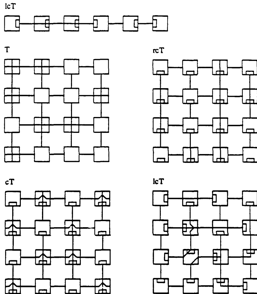
Figure 3.2: Examples of Cut-Through Communication
