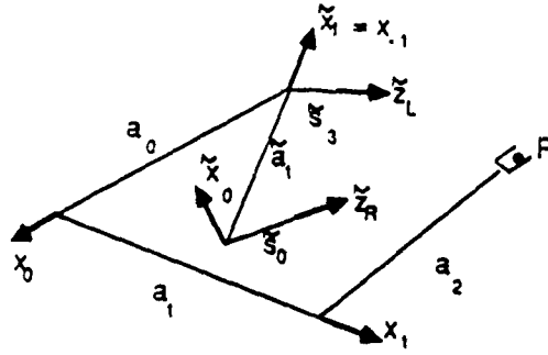
Figure 5-4: Example hand-eye system used for simulation purposes.
