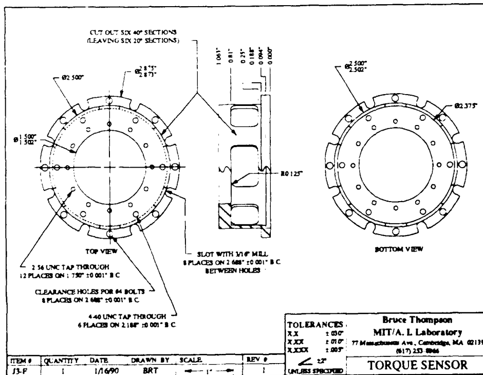
Figure A.5 Wrist Torque Sensor Engineering Drawing
