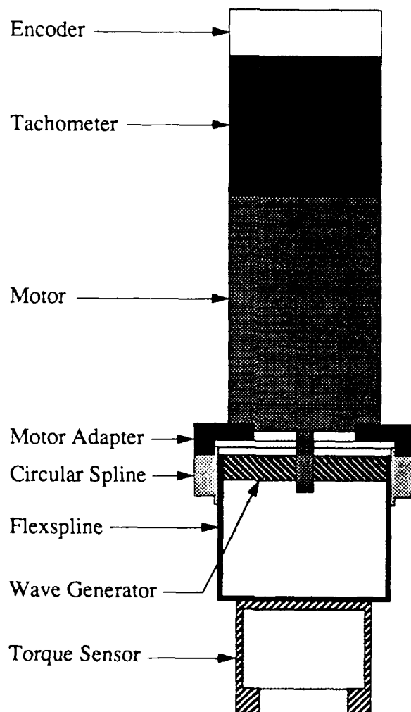
Figure 3.6a Cross Section of Elbow Drivetrain
