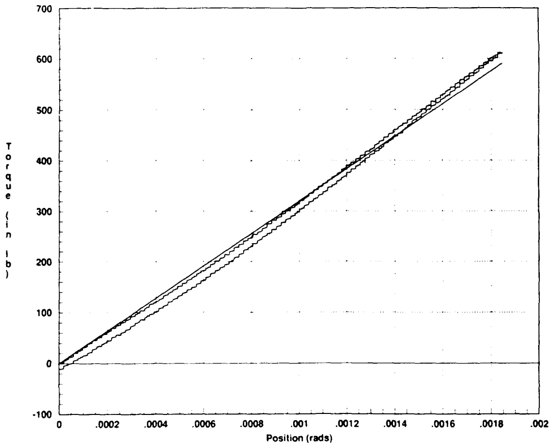
Figure 4.3 Tested H.D. Input Stiffness with Linear Approximation to Data
