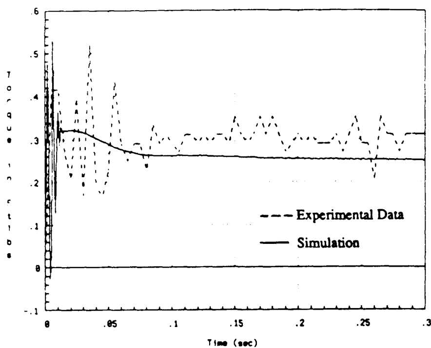
Figure 2.13 Transmission Torque Data for Toolplate Roll – Revised Motor/Amp Model
