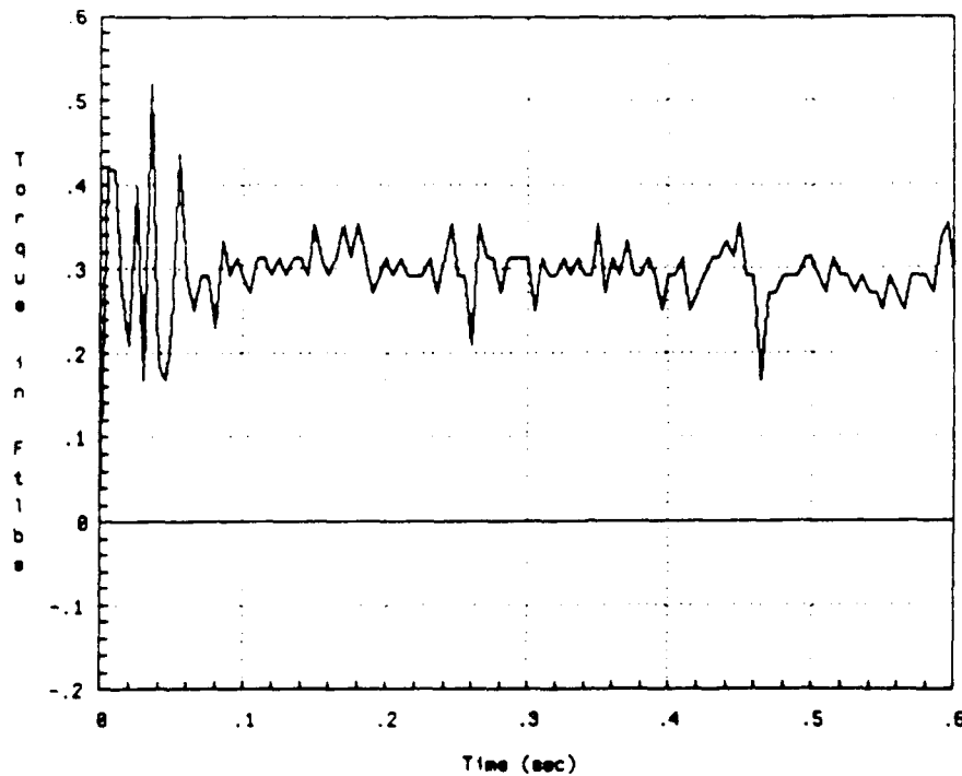
Figure 2.9 Transmission Torque Data for Toolplate Roll – Experimental Results
