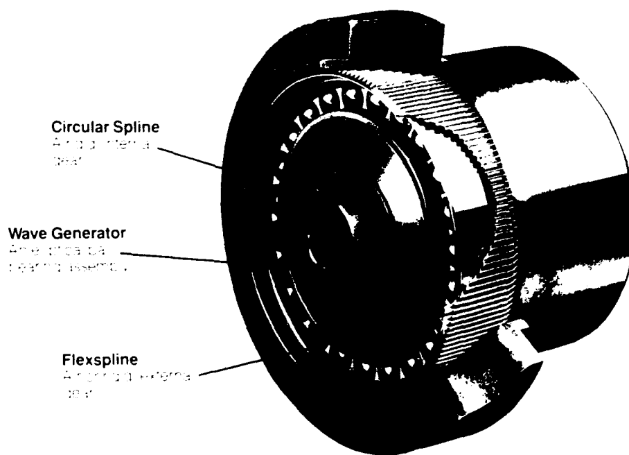
Figure 1.2 Harmonic Drive
