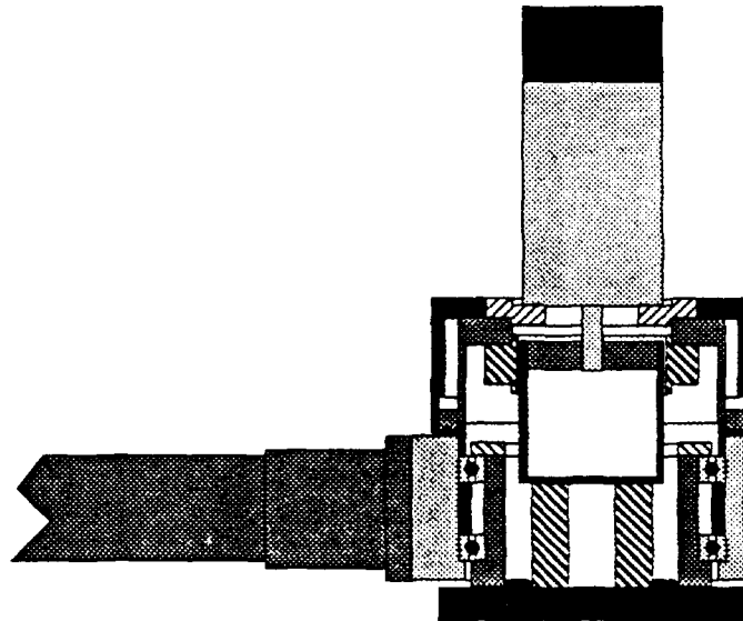
Figure 3.7b Cross Section of Assembled Wrist Joint
