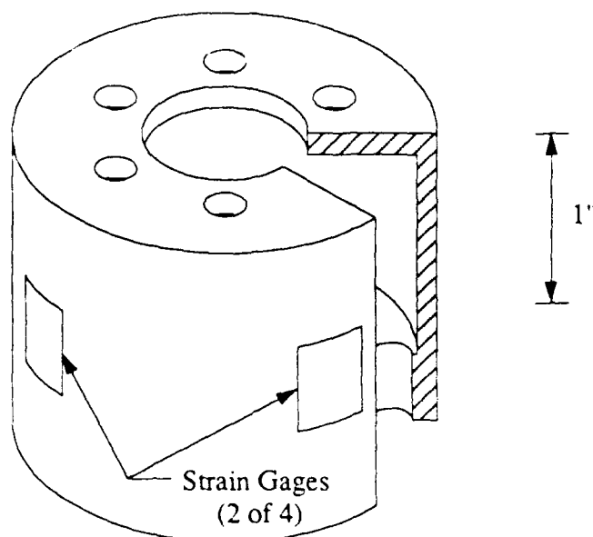
Figure 3.8 Design for the Shoulder Torque Sensor
