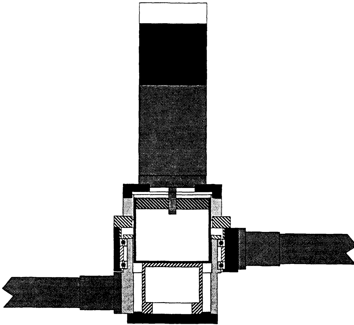
Figure 3.7a Cross Section of Assembled Elbow Joint
