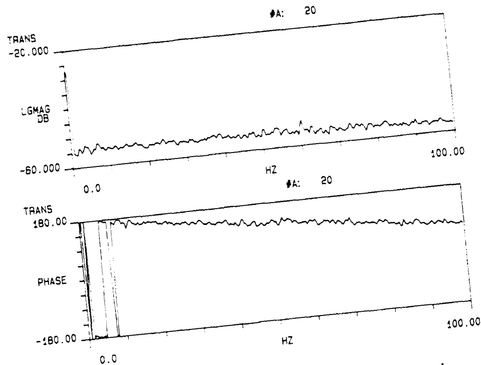
Figure 4.13 Bode Plot of System Response without Load
