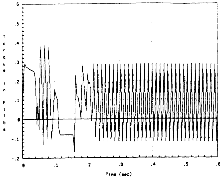
Figure 2.10 Transmission Torque Data for Toolplate Roll – Simulation Results
