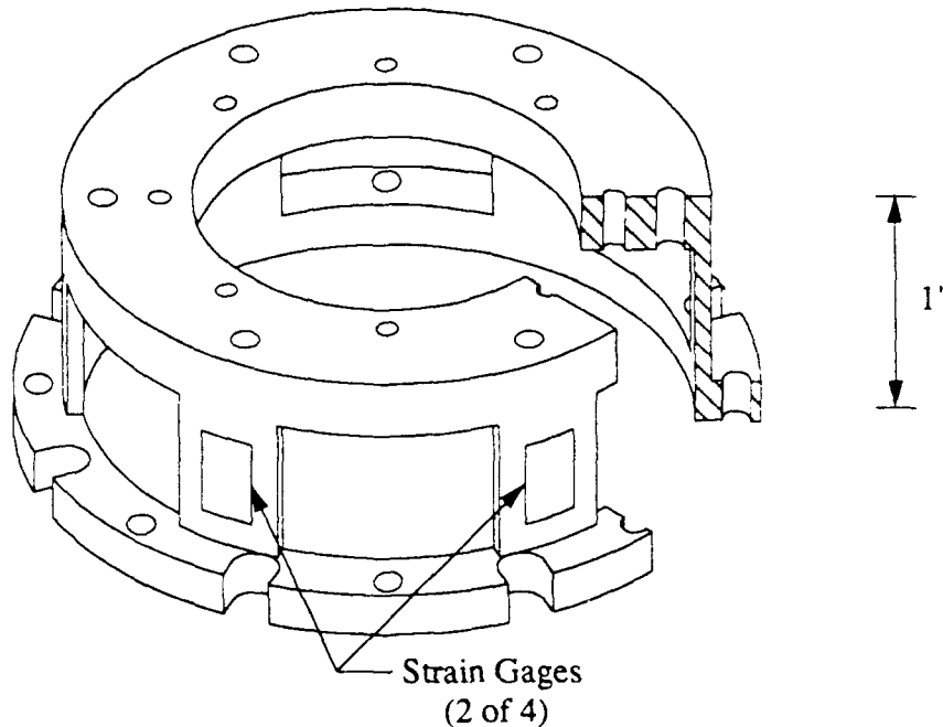
Figure 3.11 Isometric Drawing of Wrist Torque Sensor
