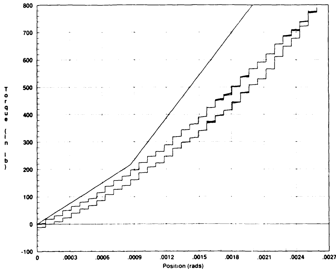
Figure 4.7 Tested H.D. Output Stiffness with Factory Quoted Stiffness
