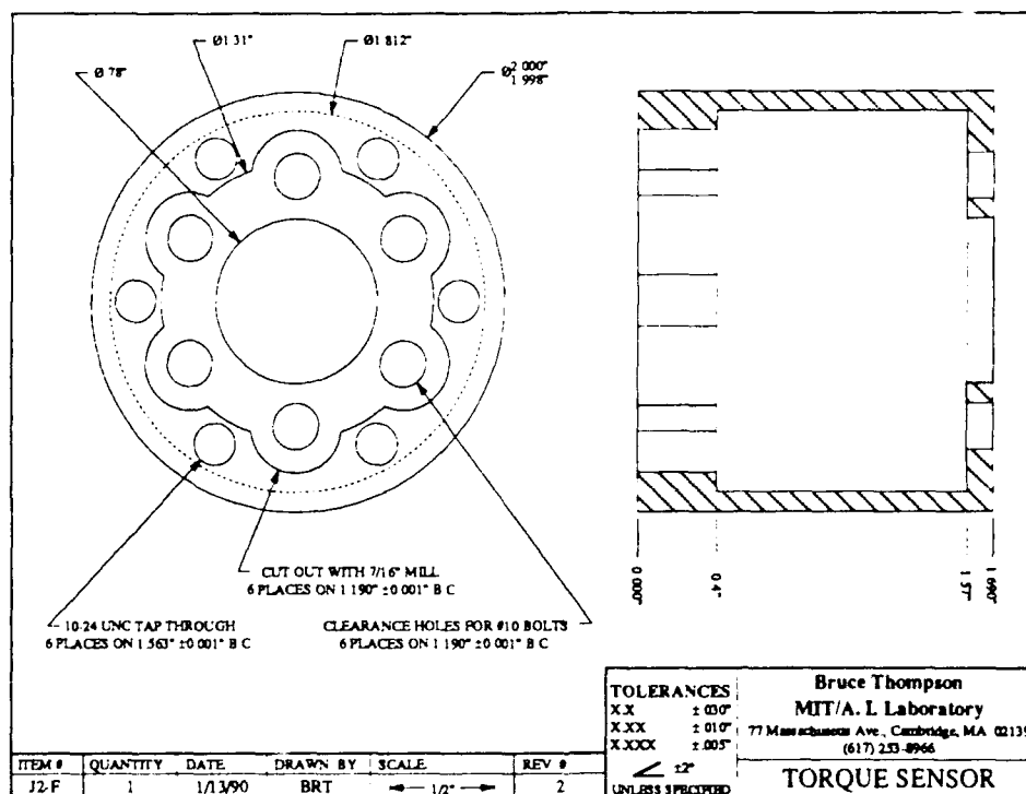
Figure A.3 Elbow Torque Sensor Engineering Drawing
