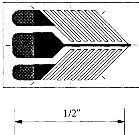
Figure 3.9 Strain Gage
