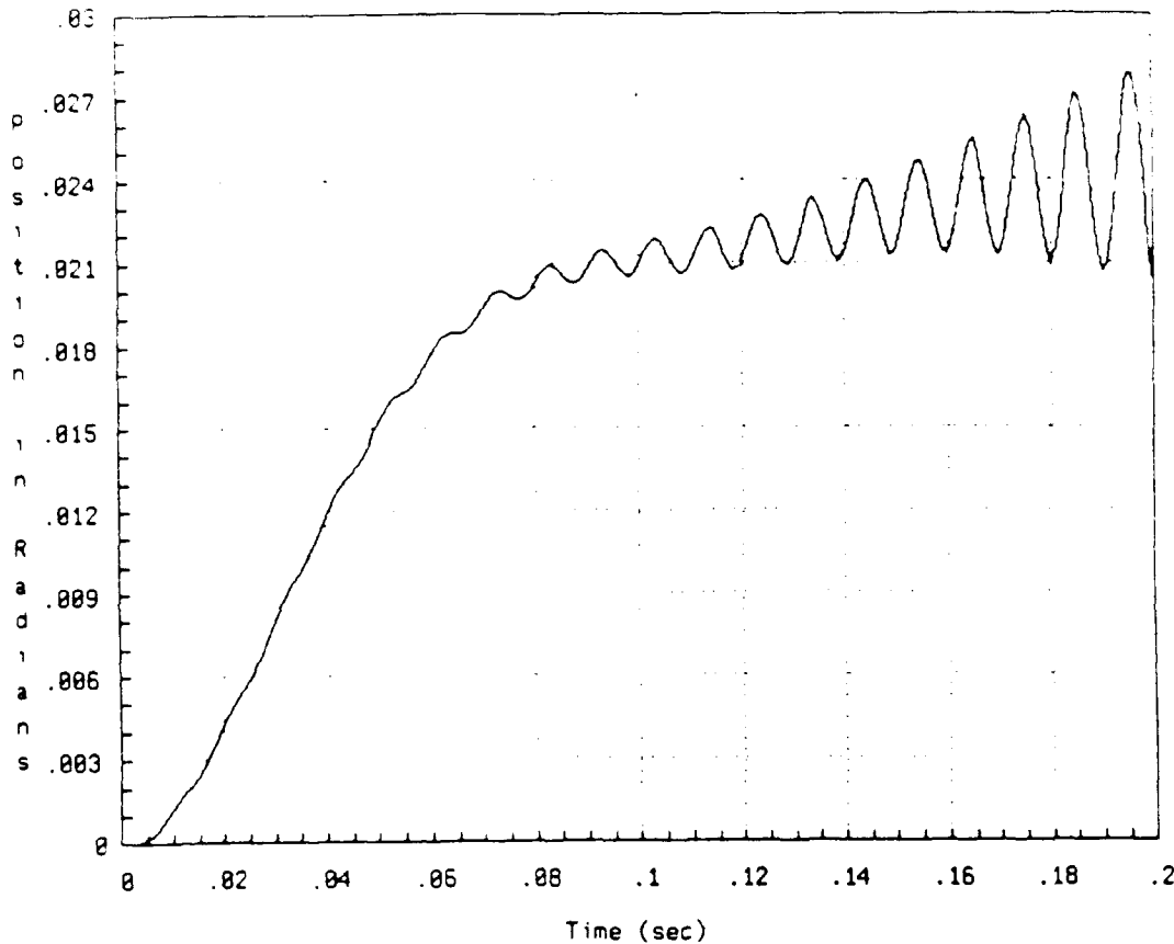
Figure 2.4 Simulated Step Response for Wrist Pitch – Linear Model
