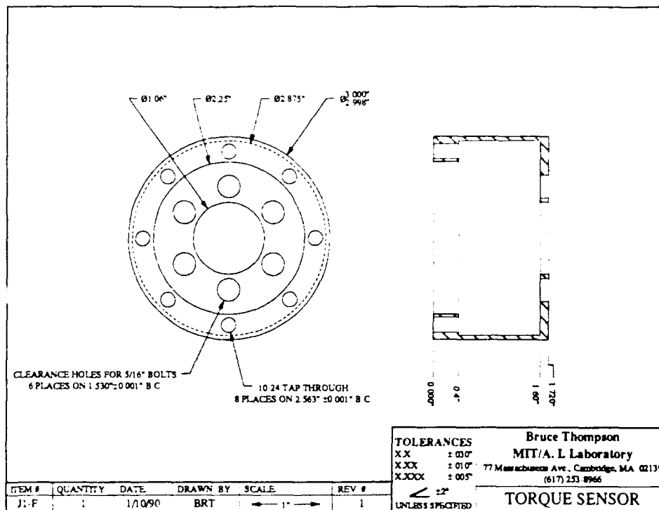
Figure A.1 Shoulder Torque Sensor Engineering Drawing
