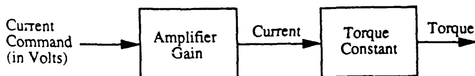
Figure 2.11 Simple Model of Amplifier and Motor
