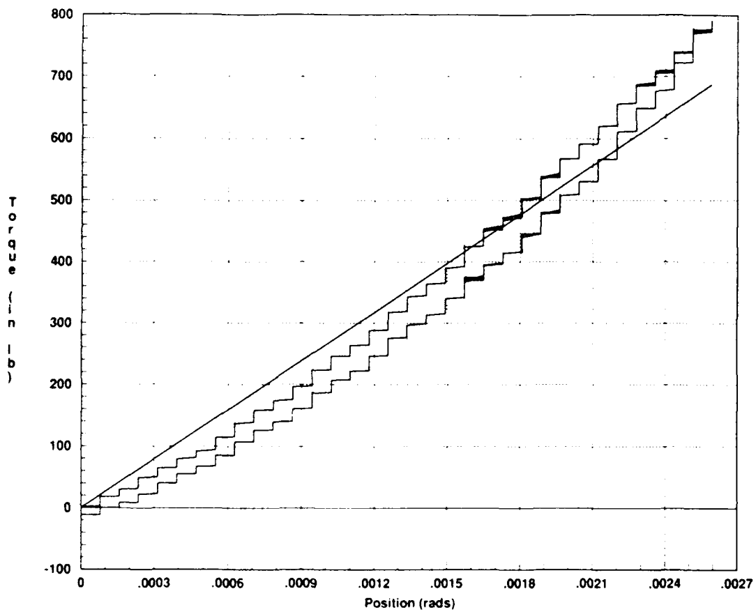
Figure 4.6 Tested H.D. Output Stiffness with Linear Approximation to Data
