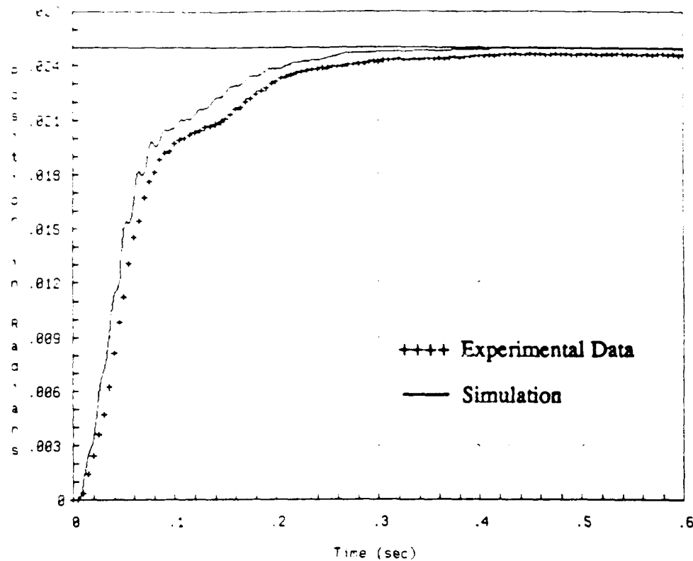
Figure 2.7 Step Response for Wrist Pitch – Non-linear Model
