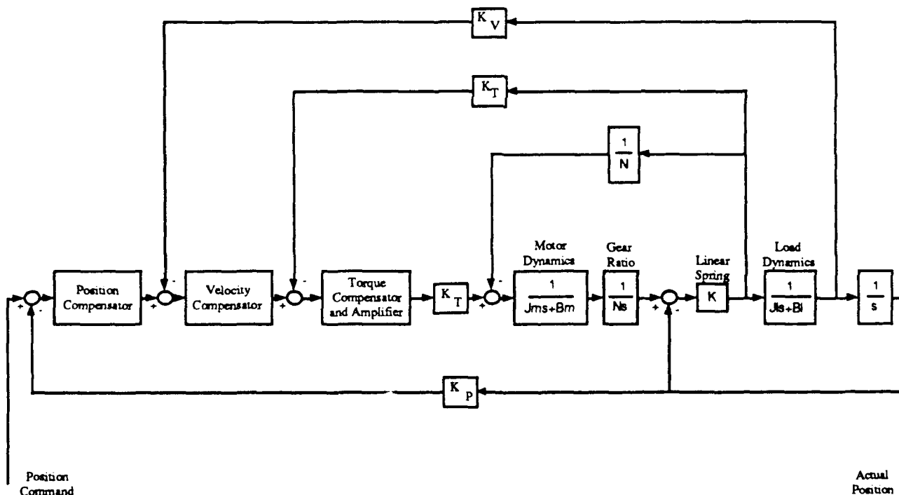
Figure 2.3 Linear Model of Typical Joint
