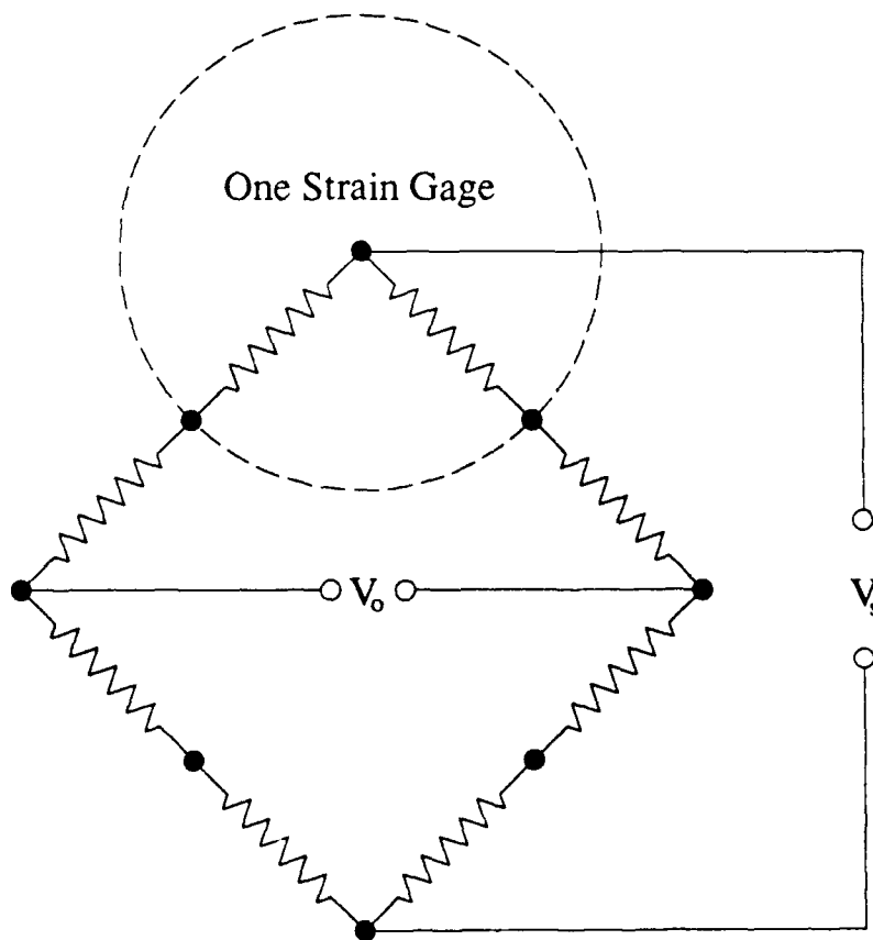
Figure 3.10 Layout for Strain Gage Wiring
