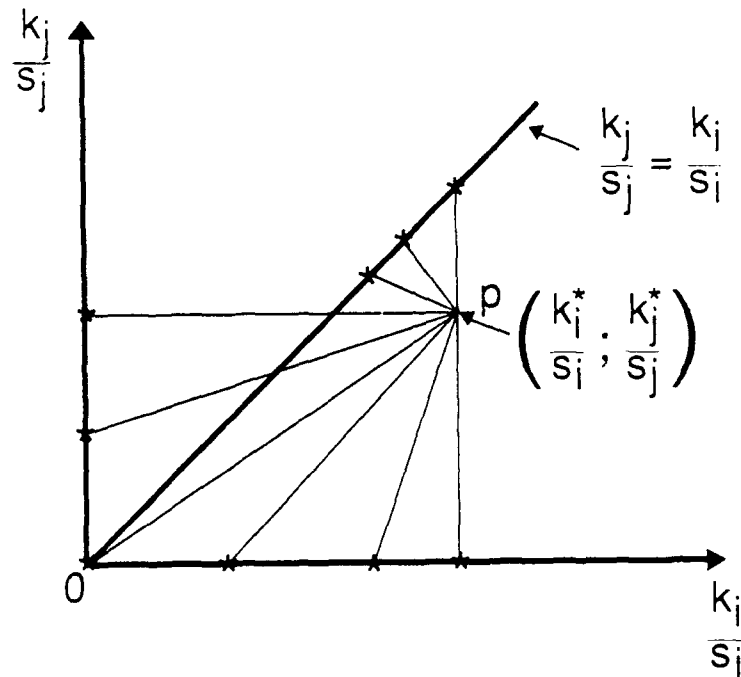
Figure 6. The minimax problem that determines the largest allowable timestep.
