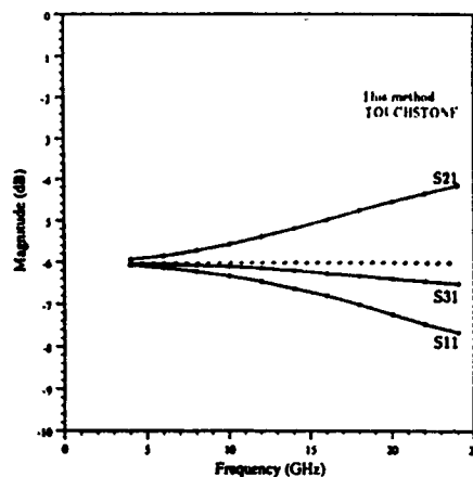
Fig. 5 Magnitude of S parameters of a right angle crossing junction ( \epsilon_r = 10.2 , h = 25 mil, w = 24 mil) Note that in TOUCHSTONE |S_{11}| = |S_{21}| \approx |S_{31}|
