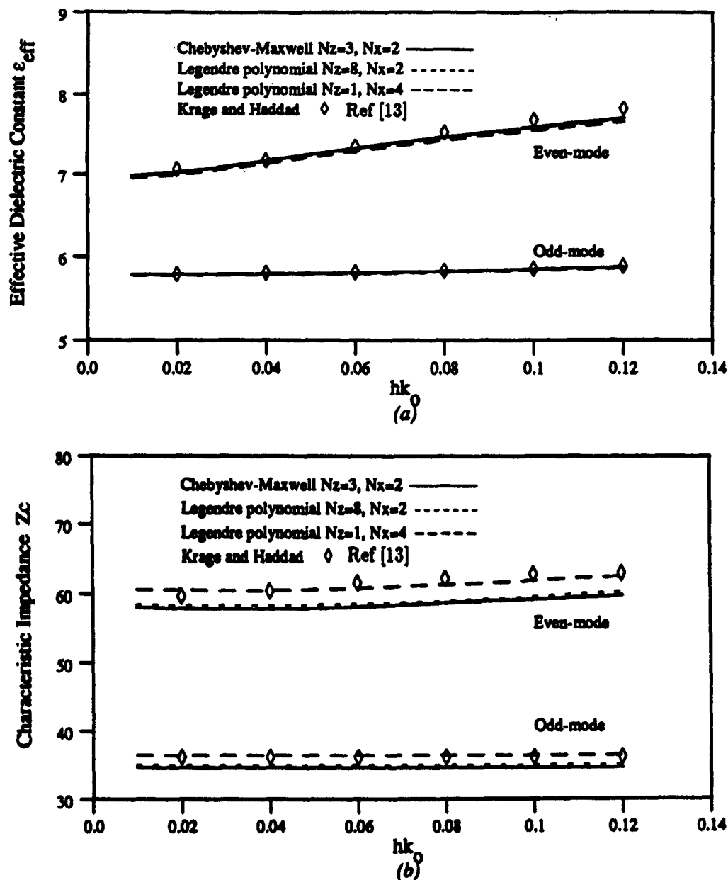
Fig. 2.11 Characteristics of symmetric coupled lines. (Fig. 2.3(c)) (a) Effective dielectric constant versus normalized frequency. (b) Characteristic impedance versus normalized frequency. \epsilon_r = 10. , \frac{A}{\lambda} = 2. , \frac{b}{\lambda} = 0.4 , \frac{w}{\lambda} = 1. , \frac{g}{\lambda} = 20.
