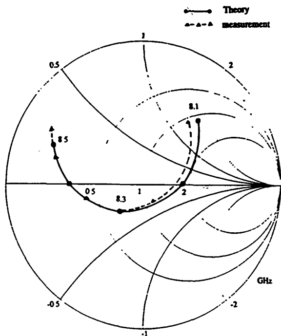
Fig. 3. Comparison between theoretical and experimental results for the input impedance of an EMC transverse dipole. \epsilon_1 = 2.17 , \epsilon_2 = 2.17 , H = 1.6 mm, B = 0.8 mm, w_1 = 1 mm, w_2 = 2.2 mm, \Delta x = 0 , \Delta s = 4.5 mm and L = 12.4 mm.
