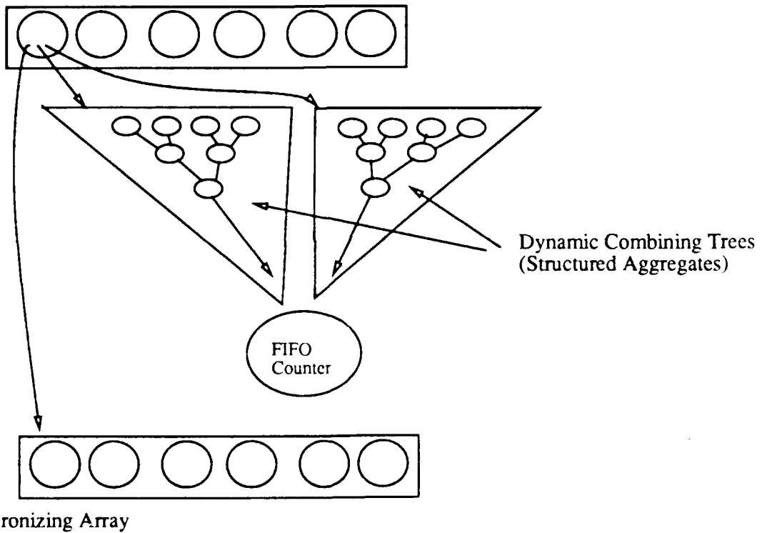
Figure 4.14: The Parallel Queue Abstraction
