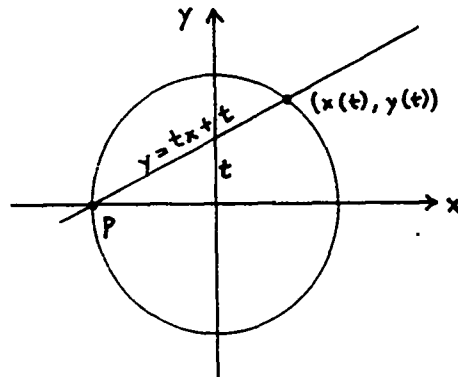
Figure 2: Parameterizing the Unit Circle
