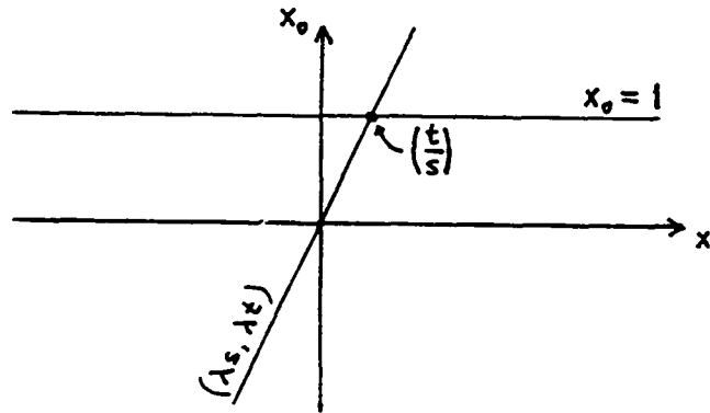
Figure 1: The Projective Line
