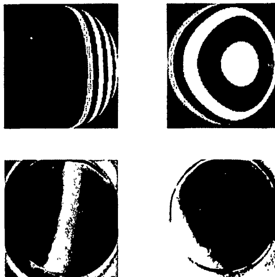
Figure 8. Comparison of the observed contours of equal apparent Doppler shift on the solar disk and contours computed from a model. Contours of equal apparent velocity on the solar surface are shown as computed (top) and recorded (bottom) at the Mt. Wilson Observatory. When the Fabry-Perot filter is tilted by about 30° relative to the solar beam, much of the rotation velocity can be removed before recording, thereby reducing the dynamic range requirement. The images on the left have no tilt; the Fabry-Perot was tilted to make the images on the right.
