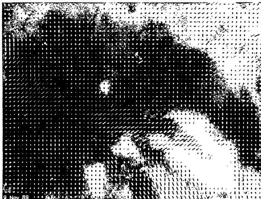
Figure 7. A map of the transverse fields obtained from the Q and U Stokes parameters as measured in a solar active region on 9 November 1989. The transverse component of the field is shown by the short line segments. The longitudinal (line-of-sight) component is represented by white and black areas for positive and negative fields, respectively.
