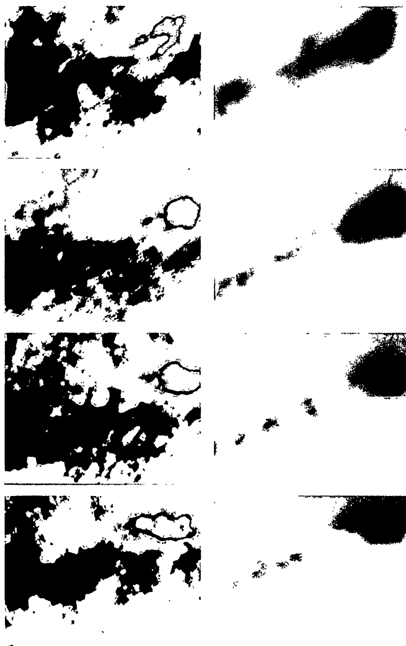
Figure 6. Daily sunspot pictures (left) and magnetic fields (right) inferred from measurements of the I and V Stokes parameters for 9-12 November 1989. These images show (top to bottom) the evolution of the active solar region and the variable quality of the data, which is caused by varying atmospheric conditions at the observatory.
