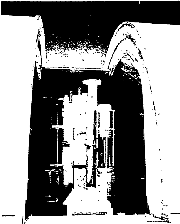
Figure 2. The APL Solar VMG (rightmost telescope) installed in the Hilltop Dome of the Sacramento Peak Observatory in Sunspot, New Mexico. The upper part is the vacuum 25-cm Cassegrain telescope. The lower part is the magnetograph optics housing.
