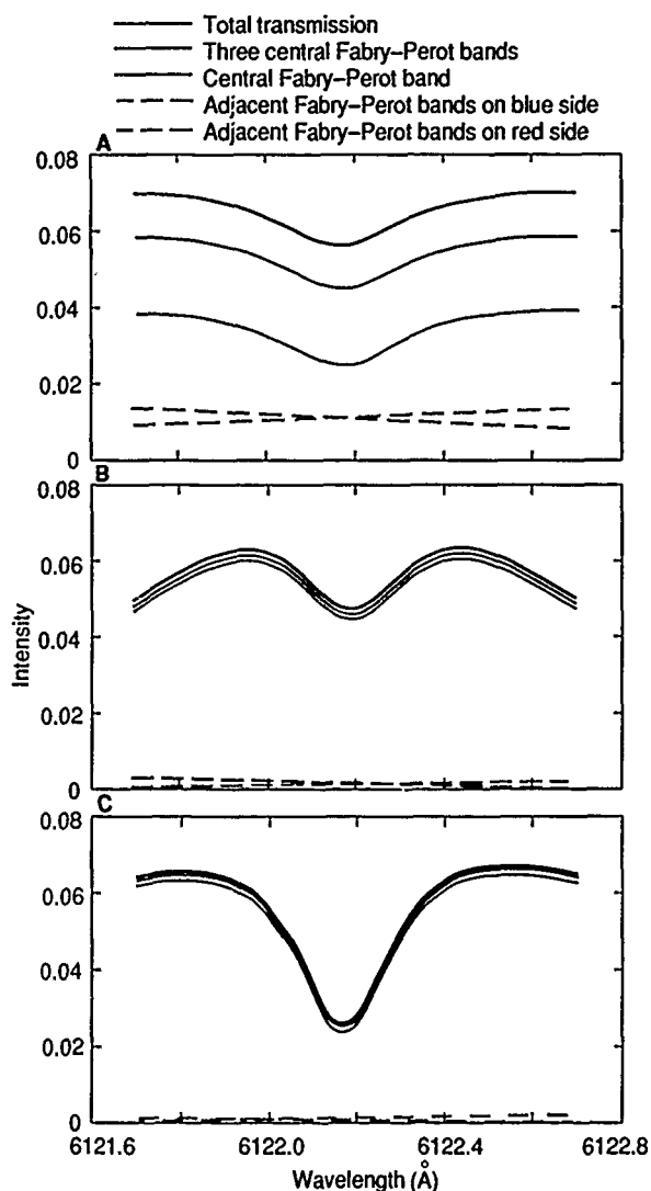
Figure 4. Comparison of spectral line profiles. A. Profiles after passage through the 0.17-Å filter and a 3.5-Å blocking filter. B. Profiles expected with the 3.5-Å blocker, a 0.17-Å Fabry-Perot filter, and a 1.1-Å cleaved mica blocker. C. Profiles expected with a 2.5-Å blocker and two lithium niobate filters (0.15- and 0.11-Å) in series.
