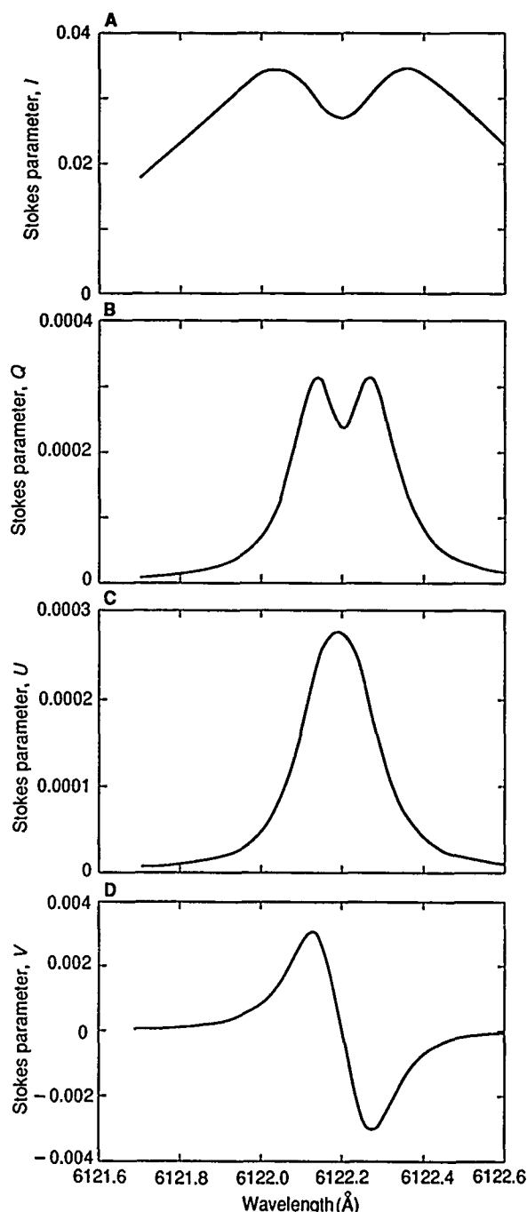
Figure 1. Simulated profiles of the Stokes parameters, which represent intensity ( I ), linear polarization ( Q and U ), and circular polarization ( V ) as functions of wavelength near the calcium line at 6122.2 \text{ \AA} in the solar spectrum. The profiles take the instrument's spectral response into account and show the magnetograph response to a 1000-G magnetic field at 30^\circ to the line of sight.
