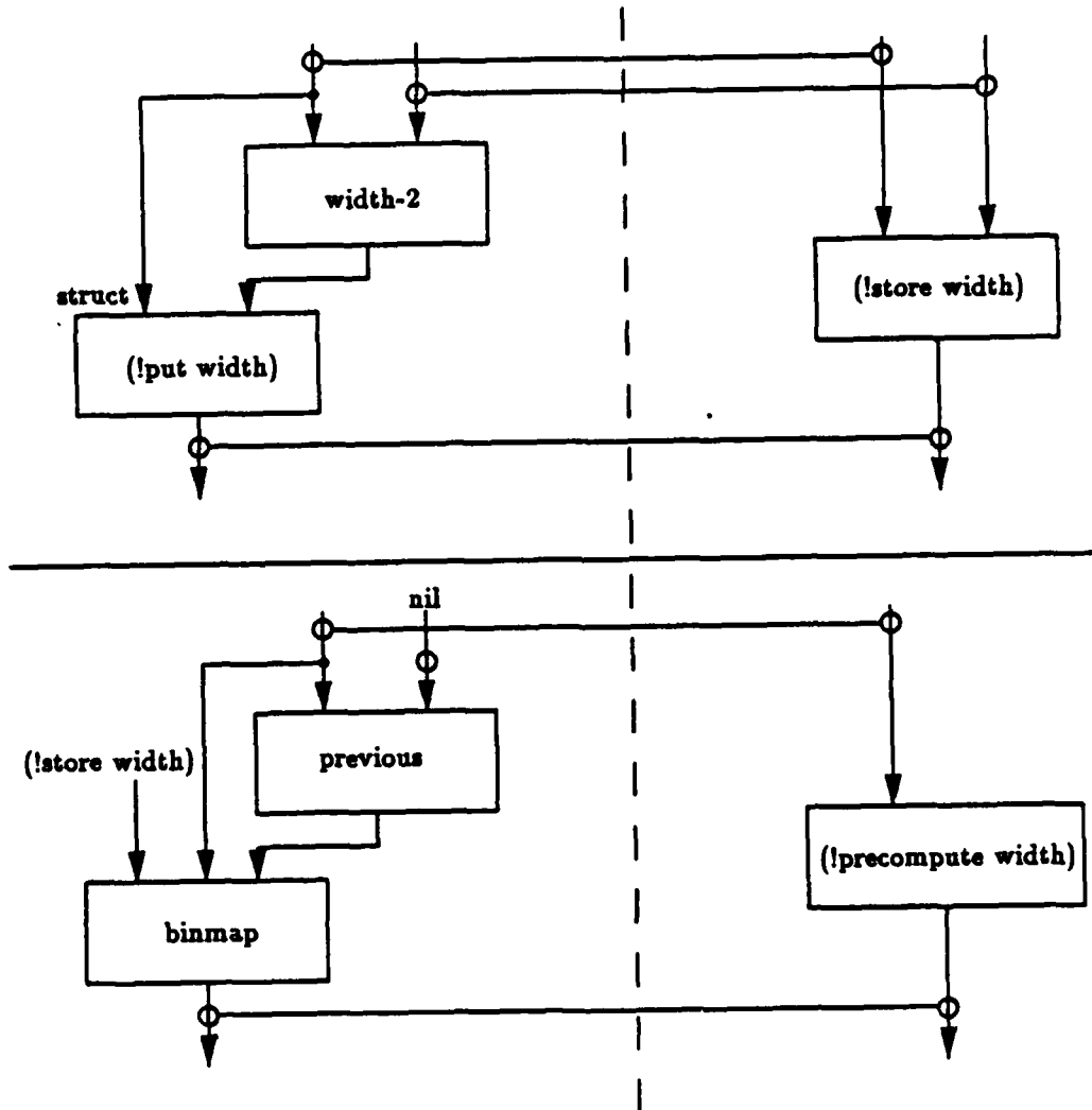
Figure 4-14: Pre-Computing the Width Mapping.
