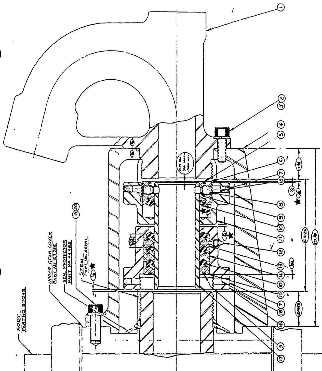
Fig. 3 BOWEN S-2.5 Power Swivel Floating Washpipe Assembly
