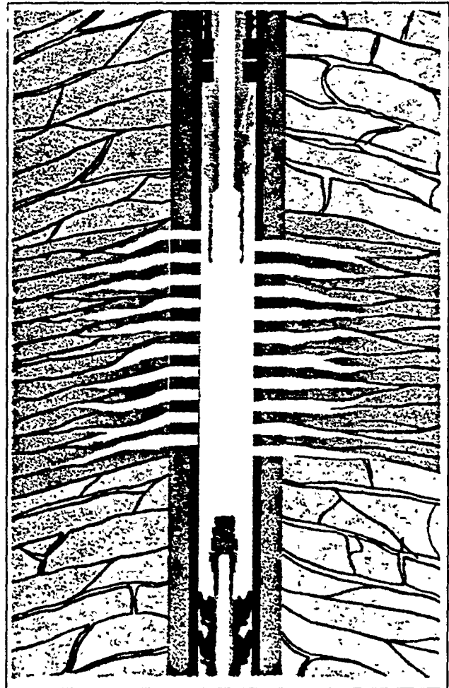
Squeeze Packer Method
